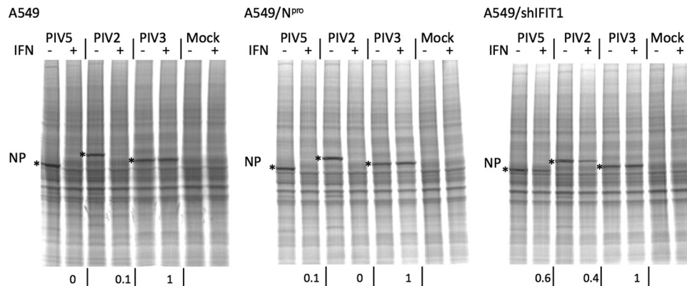
FIG 2 IFIT1 inhibits PIV5 (W3) and PIV2 (Colindale) protein synthesis but not that of PIV3 (Washington). A549, A549/N pro , and A549/shIFIT1 cells, grown in 25-cm 2 flasks were, or were not, treated with IFN 8 h prior to infection at a high MOI with PIV2, PIV3 (Washington strain), or PIV5. At 18 h p.i., cells were metabolically labeled with [ 35 S]methionine for 1 h. Total-cell extracts were separated by electrophoresis through a 4 to 12% PAG, and labeled proteins were visualized using a phosphorimager. The positions of the NP polypeptides are indicated by asterisks. The values at the bottom indicate the fraction of NP made in cells pretreated with IFN compared to untreated cells as estimated by densitometry scans.
