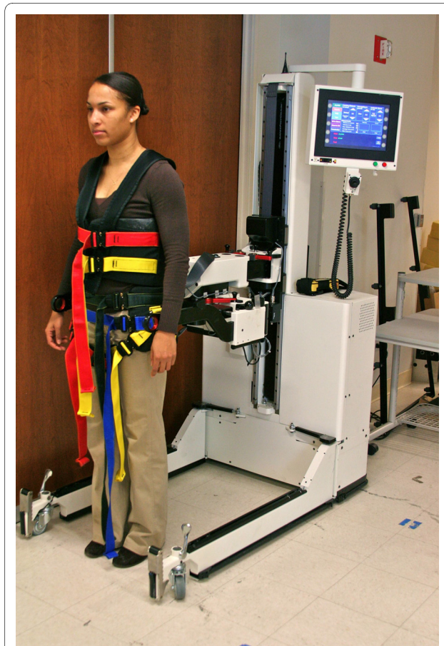
Figure 1 The KineAssist in use.
