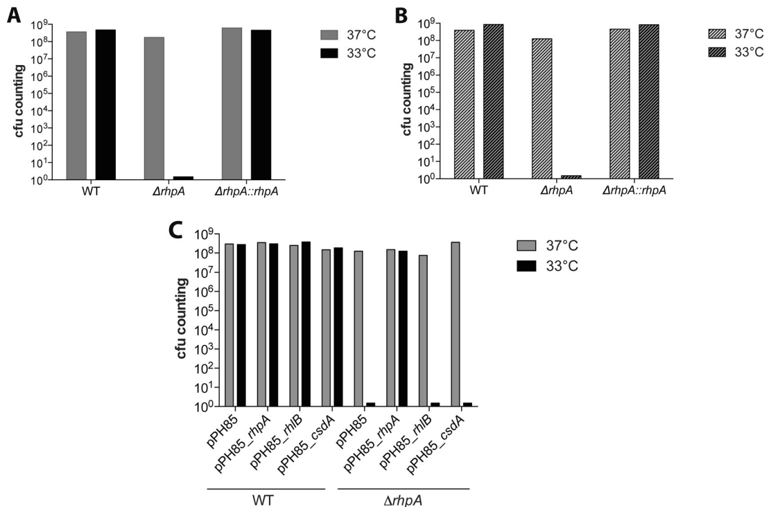
FIG 5 RhpA is essential for growth of H. pylori at 33°C and is not functionally complemented by its E. coli homologues, RhlB or CsdA. Amounts of viable bacteria of H. pylori wild-type (WT), \Delta rhpA mutant, and complemented strains were measured after incubation in BHI medium during 16 h of growth at 37°C or at 33°C. (A) Wild-type strain X47-2AL, the \Delta rhpA mutant, and the complemented mutant were incubated and colonies were enumerated on plates incubated at the same temperature (either 33°C or 37°C, as indicated). (B) Wild-type strain X47-2AL, the \Delta rhpA mutant, and the complemented mutant were first incubated at 33°C and subsequently spotted on plates at the temperature indicated in the legend, i.e., at either 33°C or 37°C. The lower temperature of 33°C completely inhibited growth of the \Delta rhpA mutant, but this growth could be rescued by subsequent incubation at 37°C. (C) Viable bacteria of H. pylori B128 wild type and of the \Delta rhpA mutant either carrying an empty vector (pPH85) or a vector expressing csdA , rhlB , or rhpA under control of an IPTG-inducible vector were enumerated. Strains were plated on blood agar medium and incubated at either 33°C or 37°C for 5 days. The lower temperature inhibited \Delta rhpA mutant growth on plates, and growth was restored when rhpA was expressed from a plasmid (pPH85_ rhpA ). Neither CsdA nor RhlB was able to rescue the cold-sensitive phenotype of the \Delta rhpA mutant strain at 33°C (see also Fig. S4).
