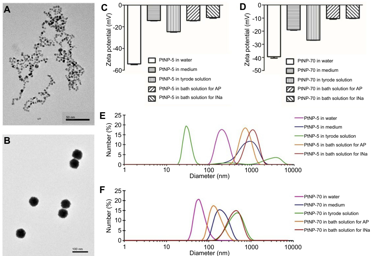
Figure 1 The morphology and characterization of PtNPs. (A and B) Transmission electron microscopy (TEM) images of PtNP-5 and PtNP-70 in the culture medium, respectively. (C and D) Zeta potentials, respectively, for PtNP-5 and PtNP-70 in different solutions 5 mins after incubation. (E and F) Hydrodynamic diameters, respectively, for PtNP-5 and PtNP-70 in different solutions 5 mins after incubation.
