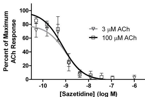
Figure 4. Sazetidine-A desensitization of the more sensitive ( \alpha 4\beta 2 ) 2 \beta 2 stoichiometry with 3 \mu\text{M} and 100 \mu\text{M} ACh. Cells stably expressing \alpha 4\beta 2 AChRs were further transfected with \beta 2 subunits and cultured in nicotine as described, to enrich for the sensitive ( \alpha 4\beta 2 ) 2 \beta 2 stoichiometry. Responses were measured with the FlexStation using a membrane potential sensitive indicator, and results were expressed as a percentage of maximum fluorescence. The responses to both 3 \mu\text{M} and 100 \mu\text{M} ACh overlapped, likely indicating that only the ( \alpha 4\beta 2 ) 2 \beta 2 stoichiometry contributes to desensitization. The plateau on the desensitization curve with sazetidine-A on mixed stoichiometries of \alpha 4\beta 2^* (shown in Figure 3) indicates that the ( \alpha 4\beta 2 ) 2 \alpha 4 stoichiometry is not desensitized even at high concentrations of sazetidine-A. doi:10.1371/journal.pone.0079653.g004
