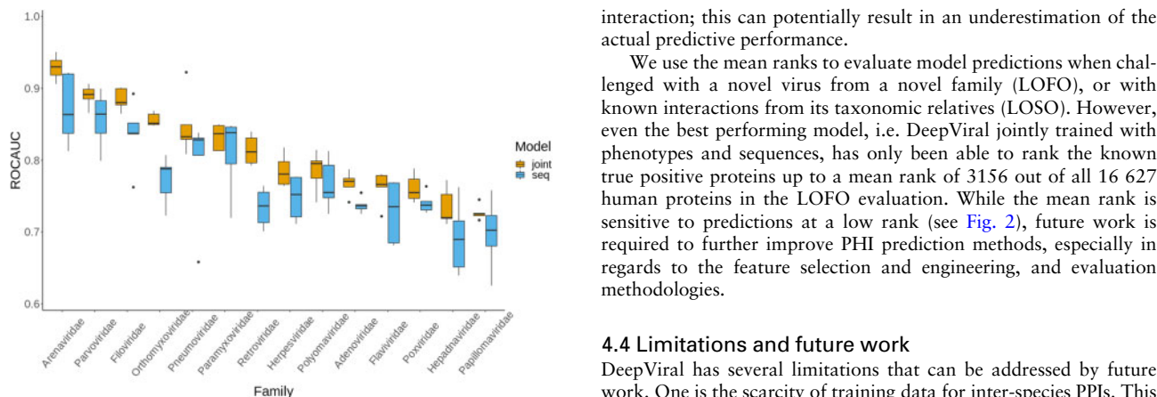
Fig. 3. ROCAUC for each of the 14 virus families from the joint model and the sequence model, respectively, ordered by the ROCAUC of the joint model
