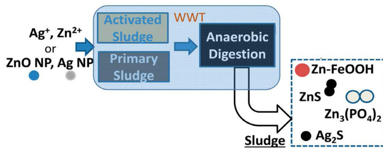
Figure 1. Similar transformation of dissolved, bulk or nanosized metals ( \text{ZnO} and \text{Ag} ) in the wastewater treatment plant (WWTP). X-ray absorption spectroscopy revealed that dissolved, bulk or nanosized \text{ZnO} and \text{Ag} particles are transformed to sulfide and phosphate minerals. \text{Zn} was also bound to iron oxohydroxides. Reprinted with permission from Ma et al. , 2014. Copyright 2014, American Chemical Society.
