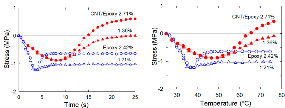
Figure 3. Time–dependent (left) and temperature–dependent (right) variations in stress during a heating of the MWCNT nanopaper/epoxy and epoxy strips from the temperature of 25 °C to 75 °C at the fixed strain denoted in the graphs.
