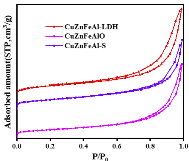
Fig. 3 N 2 adsorption-desorption isotherms of different adsorbents.
