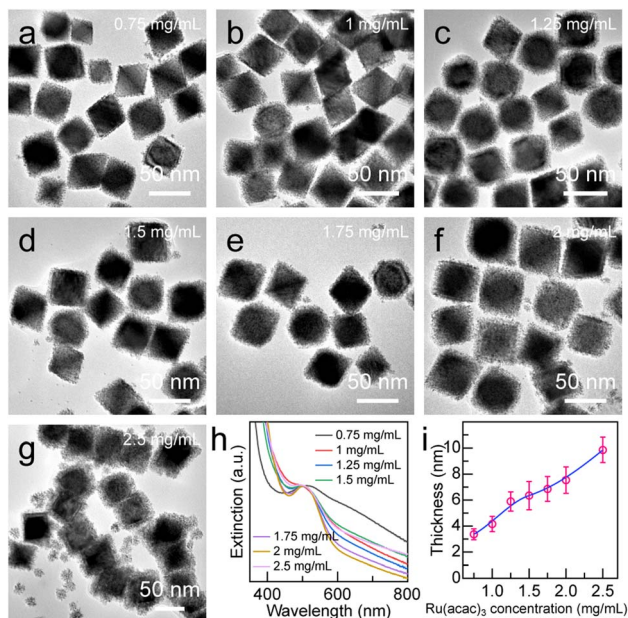
Fig. 4 Effect of precursor concentration on Ru shell thickness. (a–g) Representative TEM images of the Pd octahedron/Ru array nanostructures produced at different Ru(acac) 3 concentrations. (h) Extinction spectra of the Pd octahedron/Ru array nanostructures obtained when different Ru(acac) 3 concentrations were employed for Ru shell growth. (i) Ru shell thickness as a function of Ru(acac) 3 concentration.
