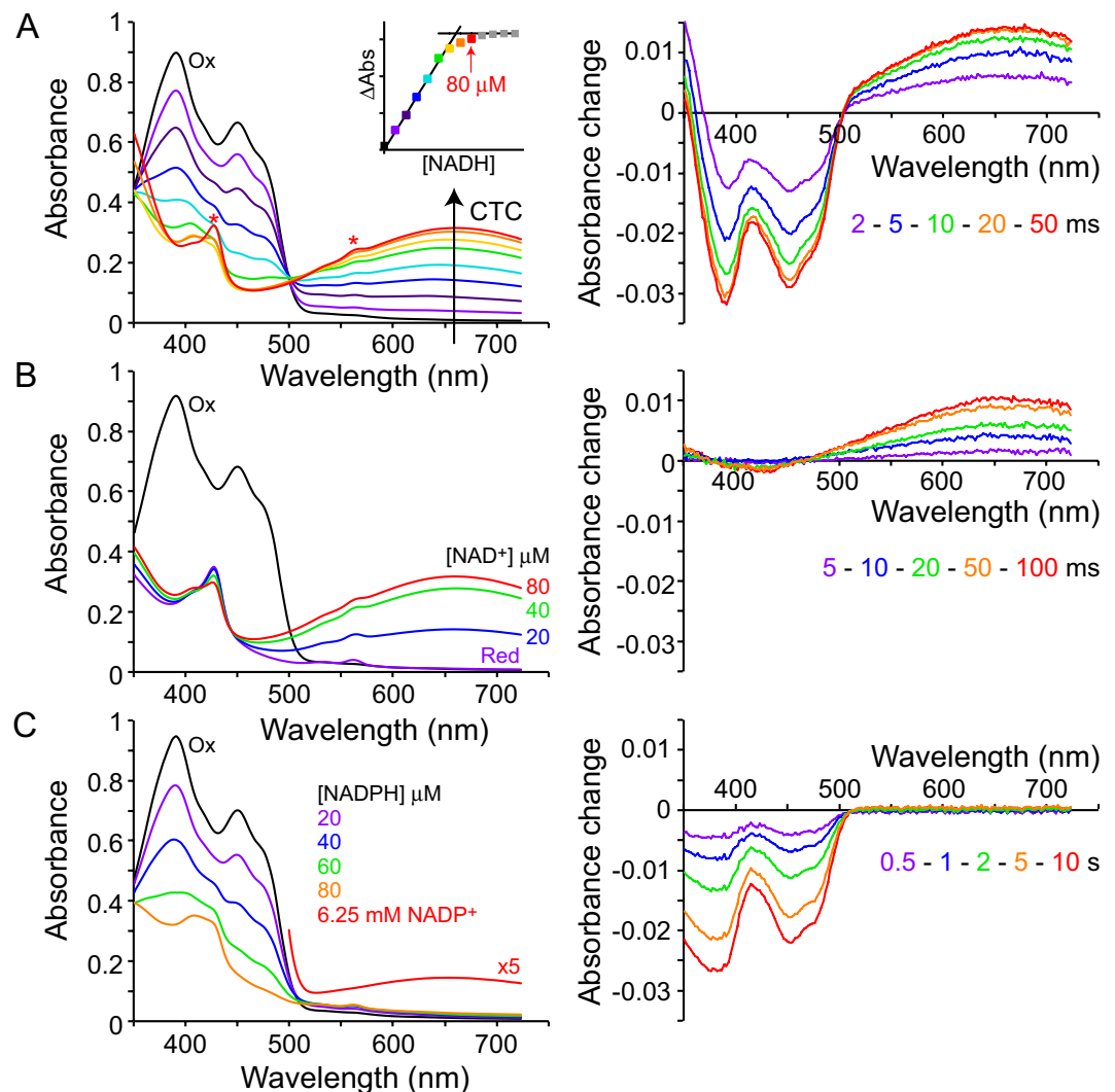
Figure 2. Spectra of NDH-2 in different redox and nucleotide-bound states. (A) Left, the spectrum of \sim 70 \mu M oxidized NDH-2 is in black (Ox), then subsequent spectra show how the spectrum evolves upon addition of 10 \mu M aliquots of NADH. Wavelengths below 500 nm show flavin reduction, wavelengths above 500 nm formation of the charge-transfer complex (CTC). The inset shows the CTC absorbance plotted against NADH concentration showing the CTC is formed close to stoichiometrically with NADH. The asterisks mark two signals from a low-level but strongly absorbing contaminant heme protein (which is estimated to be present at less than 2% of the concentration of NDH-2). Right, difference spectra (spectrum at the reported timepoint minus the oxidized spectrum) for the reaction of 4 \mu M oxidized NDH-2 with 5 \mu M NADH (concentrations after mixing) showing rapid flavin reduction and CTC formation. (B) Left, the spectrum of \sim 70 \mu M oxidized NDH-2 is in black (Ox) and that of the dithionite-reduced enzyme in violet (marked Red). Subsequent spectra follow the addition of aliquots of NAD + to generate a final spectrum equivalent to in A. Right, difference spectra (relative to the 1 ms spectrum) for the reaction of 4 \mu M dithionite-reduced NDH-2 with 4.5 \mu M NAD + (concentrations after mixing). (C) An experiment equivalent to in (A) but with NADPH instead of NADH. Left, NADPH reduces the flavin but does not form the CTC; when an extremely high concentration of NADP + is added a very weak CTC signal can be observed (for the 6.25 mM spectrum shown the 80 \mu M spectrum has been subtracted and the difference spectrum expanded by 5). Right, reduction of 4 \mu M NDH-2 by 5 \mu M NADPH (difference spectra relative to the 1 ms spectrum, concentrations after mixing) is much slower than reduction by NADH.
