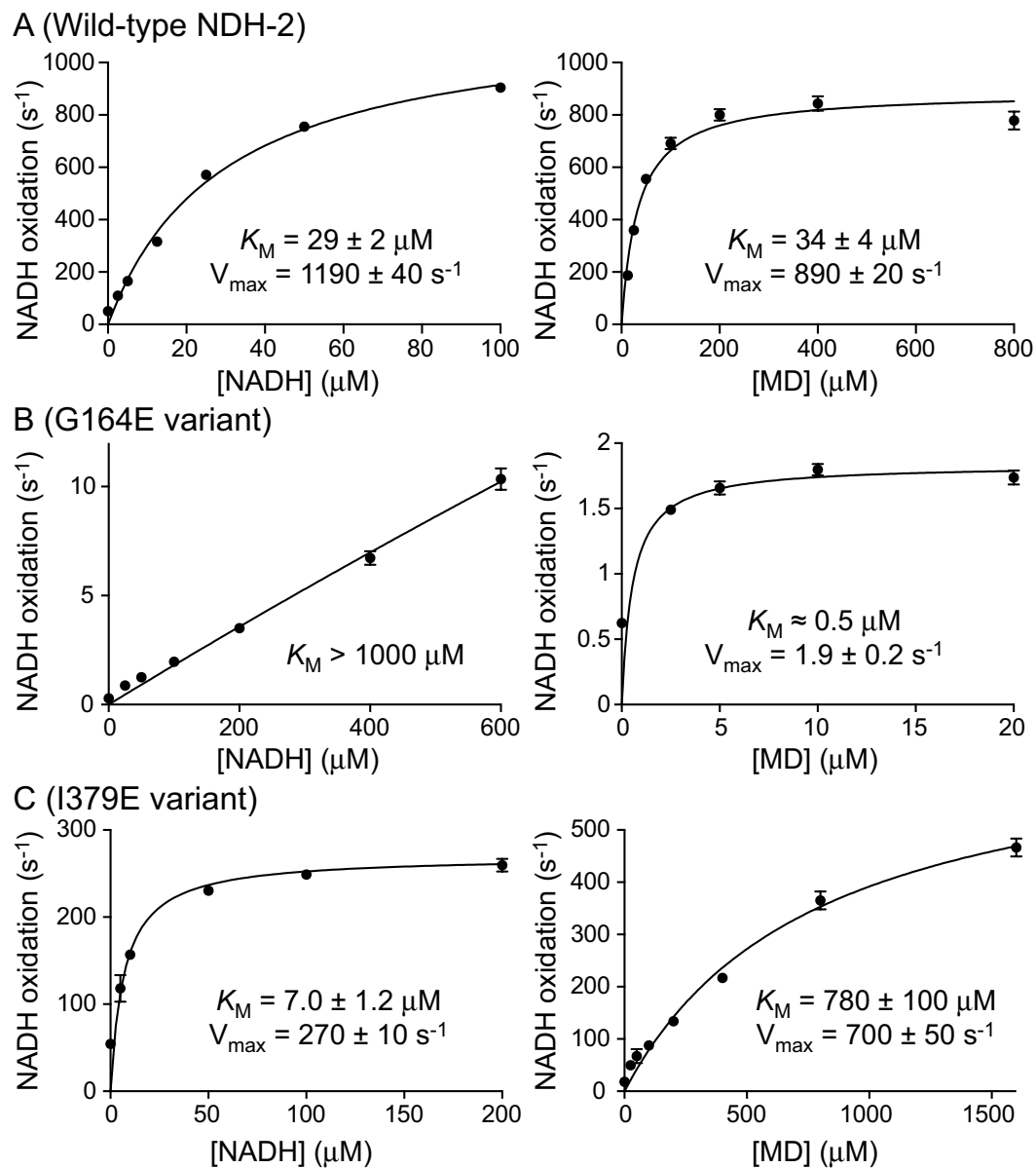
Figure 5. Steady-state kinetic data comparing the wild-type enzyme and NDH-2 variants. Measurements made with varying NADH concentrations used 400 \mu M menadione, and measurements with varying menadione concentrations used 100 \mu M NADH. The data were fit to the Michaelis-Menten equation. The data points are average values from three technical replicates with error bars \pm SEM ( n = 3 ).
