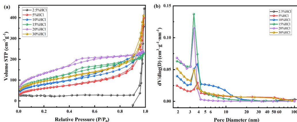
Fig. 8 \text{N}_2 adsorption desorption isotherm (a) and pore size distribution (b) of kaliophilite calcined at 900\text{ }^\circ\text{C} after treatment with different concentrations of HCl (2.5–30%) at 80\text{ }^\circ\text{C} .
