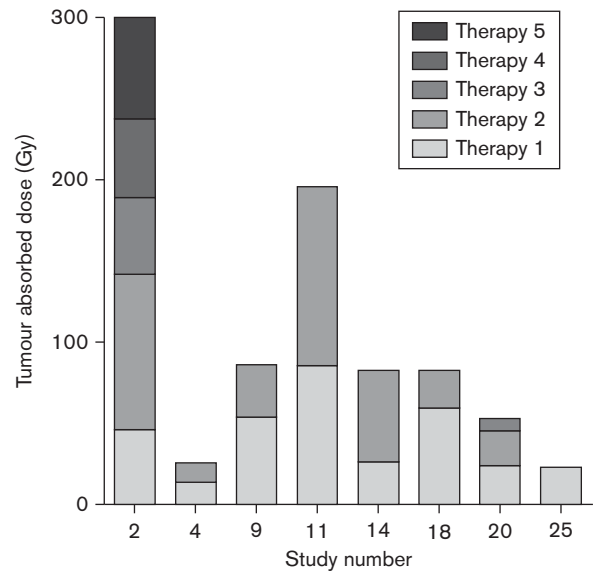
Tumour-absorbed doses.
