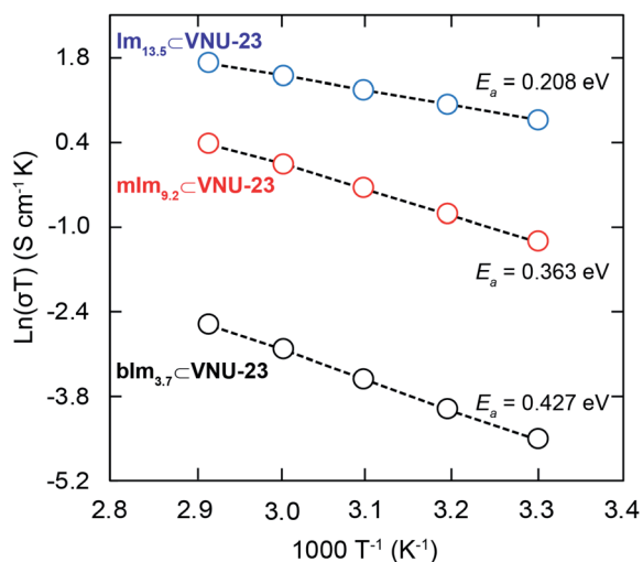
Fig. 7 Temperature-dependent proton conductivity measurements (30–70 °C) under 85% RH for \text{Im}_{13.5}@VNU-23 (blue), \text{mIm}_{9.2}@VNU-23 (red), and \text{bIm}_{3.7}@VNU-23 (black).
