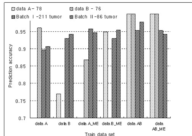
Figure 4 Comparison of the prediction accuracies between the proposed method and the ME method.
