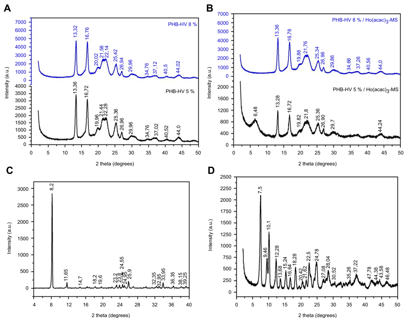
Figure 9 X-ray diffractograms of: (A) raw PHB-HV, (B) PHB-HV loaded with Ho(acac) 3 -MS, (C) Ho(acac) 3 -crystalline, and (D) Ho(acac) 3 -amorphous. Abbreviations: PHB-HV, poly(3-hydroxi-butyrate-co-3-hydroxy-valerate); MS, microspheres.
