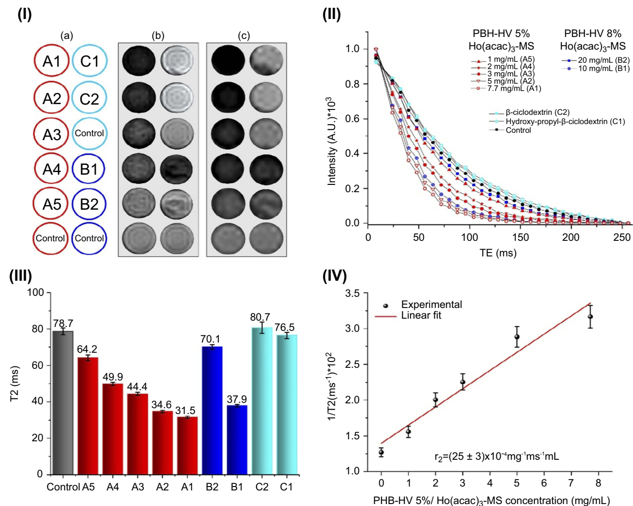
Figure 12 Relaxometry characterization of the PHB-HV microparticles loaded with holmium acetylacetonate. (I) Schematic drawing of samples (A) microsphere added (A1) 7.7 mg; (A2) 5.0 mg; (A3) 3.0 mg; (A4) 2.0 mg; and (A5) 1.0 mg. PHB-HV 8%/Ho(acac) 3 -MS, mass of microsphere added (B1) 20 mg; (B2) 10 mg. Inclusion complex of β-cyclodextrin and Ho(acac) 3 , initial concentration of 9.12 \times 10^{-3} \text{ mol L}^{-1} (C1), and hydroxy-propyl-β-cyclodextrin and Ho(acac) 3 , initial concentration of 1.94 \times 10^{-3} \text{ mol L}^{-1} (C1). (B) T_2 and (C) T_2^* weighted MRI of the corresponding samples indicated in (A). (II) Curves of MRI signal intensity of the samples indicated in (A) in the function of TEs. (III) T_2 values determined from the curves showed in item (II). (IV) Calculation of the value of r_2 from the linear correlation between the inverse of the T_2 values of the samples (A1–A5) and the concentrations of the corresponding microparticles.
