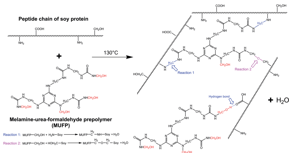
Fig. 5 Cross-linking reaction process between the soy protein isolate and melamine-urea-formaldehyde prepolymer (MUFPP).
