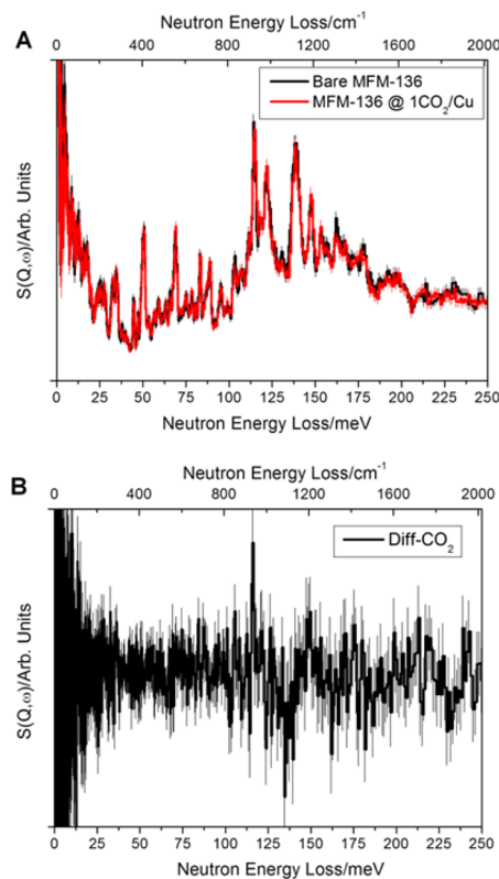
Figure 4. (a) Overlay of the INS spectra for bare and \text{CO}_2 -loaded MFM-136; (b) difference INS spectrum for the bare and \text{CO}_2 -loaded MFM-136.
