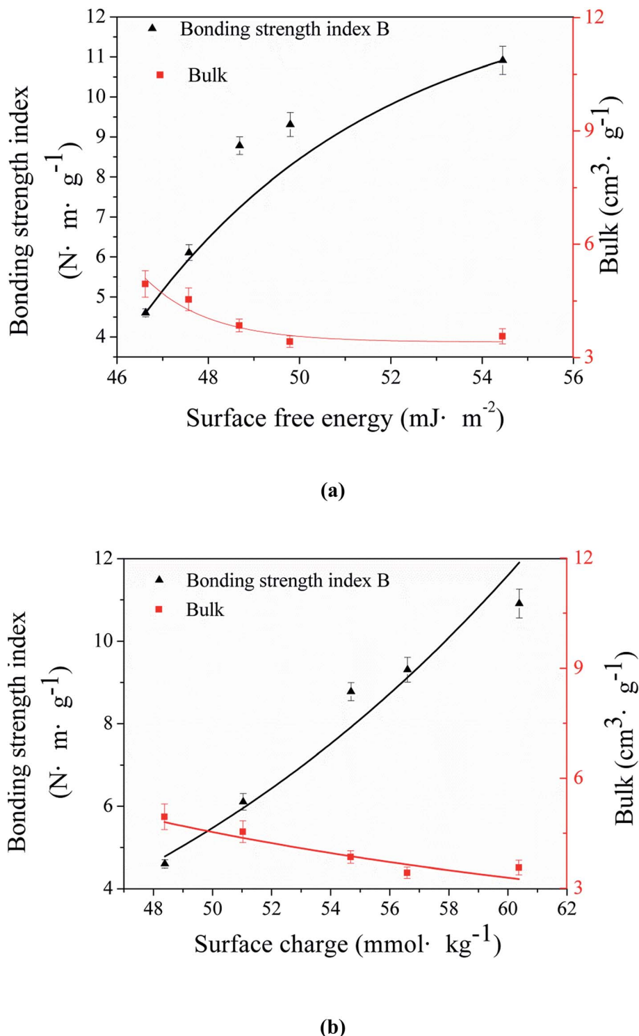
Fig. 6 Relationship between fiber surface wettability and bonding strength index and the bulk.
