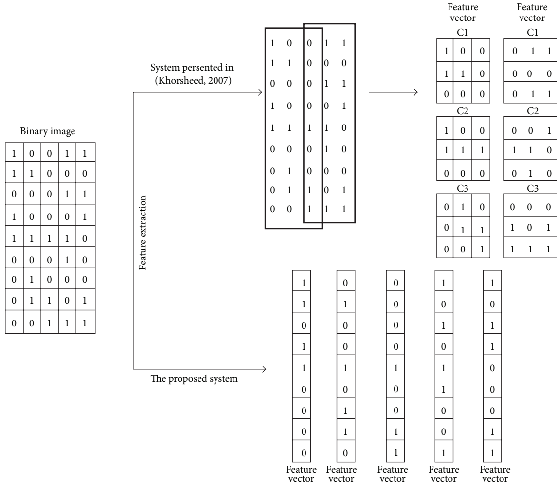
FIGURE 5: Feature extraction using the proposed algorithm and Khorsheed [7].
