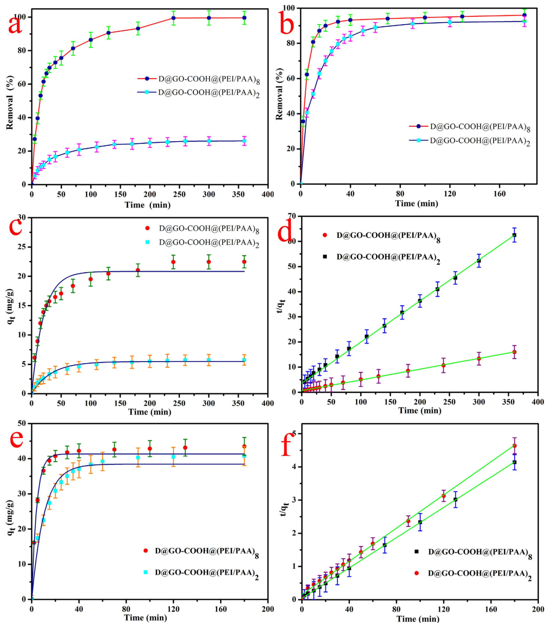
Figure 9. The percent dye removal rate versus time plots and adsorption kinetics curves of as-prepared D@GO-COOH@(PEI/PAA) 2 and D@GO-COOH@(PEI/PAA) 8 composites on RhB (a,c,d), and MB (b,e,f) at 298 K.
