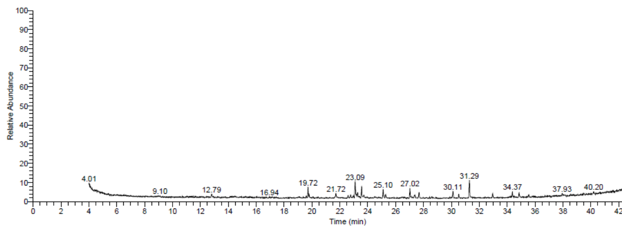
Supplementary Figure 2. GC-MS analysis of L. pruinosum extract
