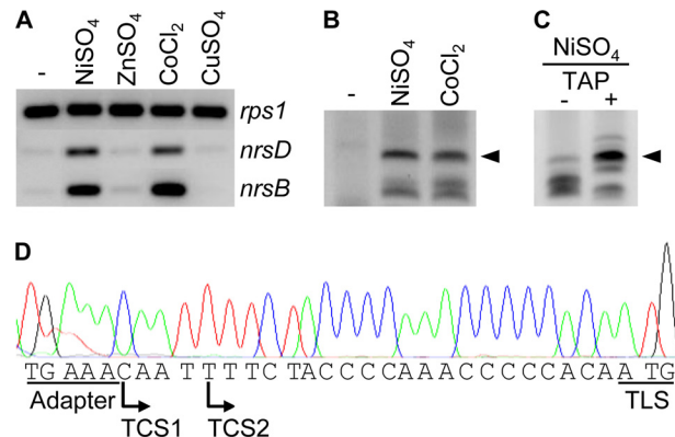
FIGURE 3. RLM-RACE identifies Ni(II)- and Co(II)-responsive transcription start sites in the nrsC-nrsD intergenic region. A , RT-PCR analysis of nrsD , nrsB , and rps1 transcript abundance in WT and \Delta inrS in response to maximum noninhibitory concentrations of four metal salts. B , RLM-RACE using RNA from WT cells exposed to maximum noninhibitory concentrations of NiSO 4 and CoCl 2 . C , separate RLM-RACE experiment with RNA extracted from Ni(II)-treated cells in which tobacco acid pyrophosphatase treatment was omitted from the control sample. The indicated products are of the expected size (~400 bp) for transcripts originating from an nrsD promoter. The abundance of the ~400 bp PCR products increase in a tobacco acid pyrophosphatase (TAP)-dependent manner. D , the ~400-bp products were cloned, sequenced, and the 3' end of the adapter is indicated along with transcriptional start site (TCS1) and the translational start site (TLS). A separate RLM-RACE experiment identified an alternate transcriptional start site (TCS2) 4 bp downstream of TCS1.
