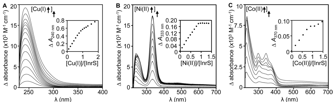
FIGURE 1. Cu(I), Ni(II), and Co(II) bind to InrS with spectral features more similar to CsoR than RcnR. Apo-subtracted UV-visible difference spectra of InrS titrated with A , Cu(I), B , Ni(II) and C , Co(II) using 40, 10.4, and 32.7 \mu\text{M} InrS, respectively (data expressed per mole InrS monomer \text{l}^{-1} \text{cm}^{-1} ), are shown. Insets are binding isotherms at selected absorbance maxima.
