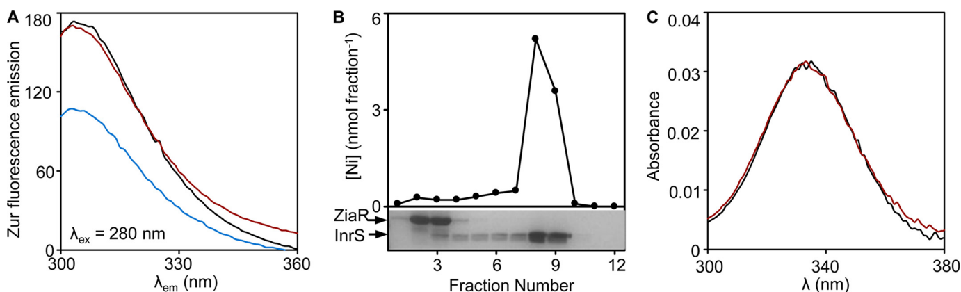
FIGURE 7. Ni(II) partitions from Zur, ZiaR, and CoaR to InrS. A , fluorescence emission spectrum of apo-Zur (10 \mu\text{M} ) (black line) and following quenching with Ni(II) (10 \mu\text{M} ) (blue line). Addition of apo-InrS (10 \mu\text{M} ) to Ni(II)-Zur fully alleviates quenching (red line). B , ZiaR (20 \mu\text{M} ) equilibrated with Ni(II) (9.5 \mu\text{M} ) before addition of apo-InrS (20 \mu\text{M} ). Proteins were separated by heparin affinity chromatography and fractions assayed for nickel by ICP-MS and protein by SDS-PAGE. C , absorption spectrum of Ni(II)-InrS (2.4 \mu\text{M} Ni(II), 5 \mu\text{M} InrS) (black line). Addition of apo-InrS (5 \mu\text{M} ) to Ni(II)-CoaR (2.4 \mu\text{M} Ni(II), 5 \mu\text{M} CoaR), which shows negligible absorbance in this region and is used as base line generates a spectrum (red line) which overlays that for 2.4 \mu\text{M} Ni(II)-InrS.
