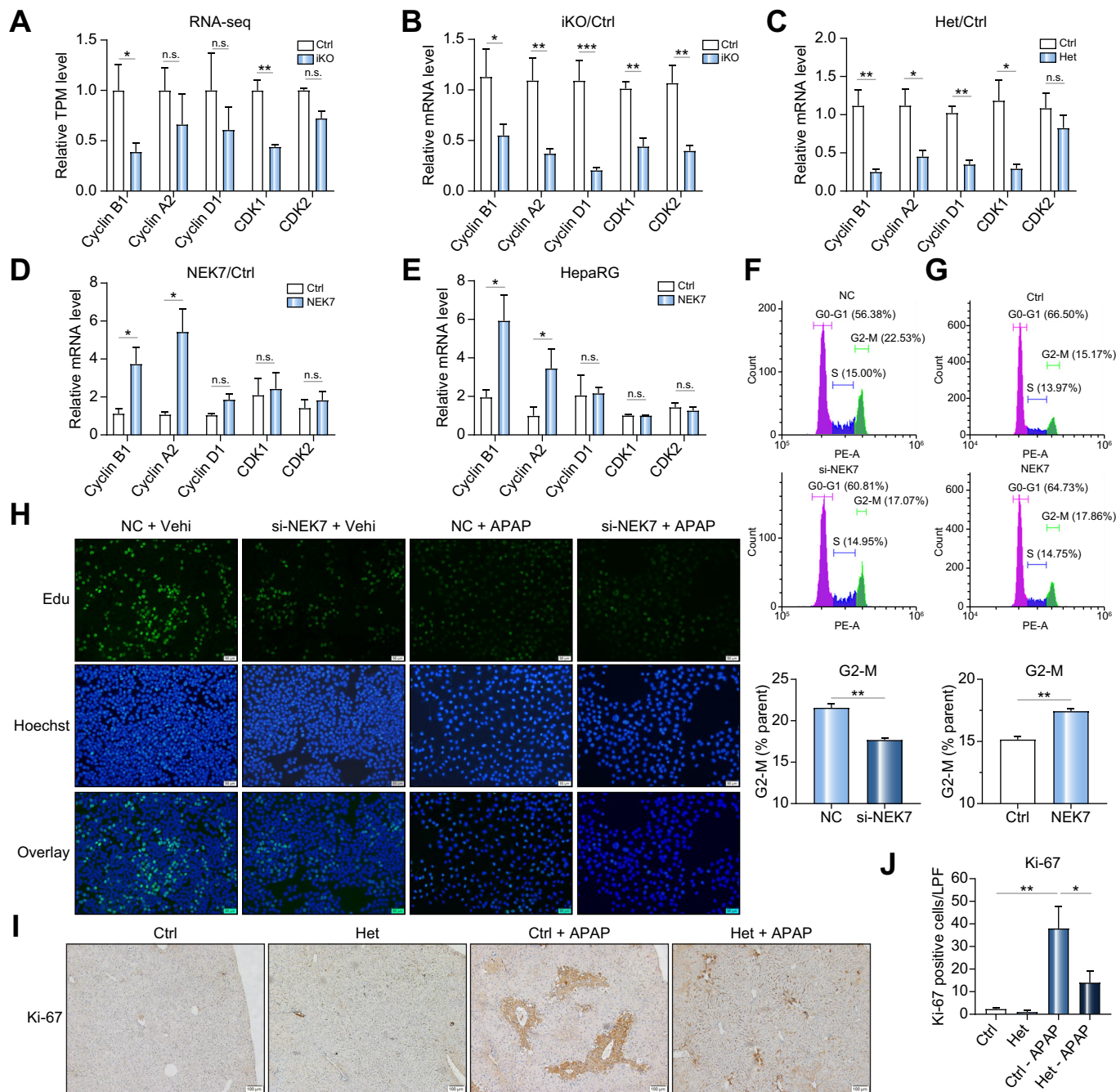
Fig. 5. Reduced NEK7 impairs cell cycle progression. (A) Relative transcript levels of cyclin B1, cyclin D1, cyclin A2, CDK1, and CDK2 profiled from the transcriptome of liver tissue (iKO mice and Ctrl mice, n = 3 ). Relative mRNA levels of cyclin B1, cyclin A2, cyclin D1, CDK1, and CDK2, (B) in the livers of iKO mice with respect to control mice (Ctrl), n = 6 , (C) in the livers of Het mice and control mice, n = 6 , (D) in NEK7 overexpressing livers and control livers, n = 6 , (E) in HepaRG cells transfected with NEK7 plasmids (NEK7) and control plasmids (Ctrl), n = 3 . (F, G) Flow cytometry analysis of the cell number in each phase of the cell cycle and quantification of the cell number in G2-M, n = 3 . (H) EdU staining showing the proliferation activity of HepaRG cells in each group, n = 3 . (I) Immunohistochemical staining of Ki-67 in liver sections; scale bars, 100 \mu\text{m} ; quantification of the positive cells, n = 3 (J). Experimental design: mice were treated with APAP or saline for 24 h. Cells were transfected with si-NEK7 or negative control for 24 h, followed by APAP or vehicle for 24 h. All values are represented as the means \pm SEM. Significant differences were analysed using a 1-way ANOVA or Student t test, * p < 0.05 , ** p < 0.01 , *** p < 0.001 . APAP, acetaminophen; Ctrl, control; Het, heterozygous; iKO, inducible knockout; NC, negative control; NEK7, NIMA-related kinase 7; n.s., no significance; TPM, transcripts per kilobase of exon model per million mapped reads; Vehi, vehicle.
