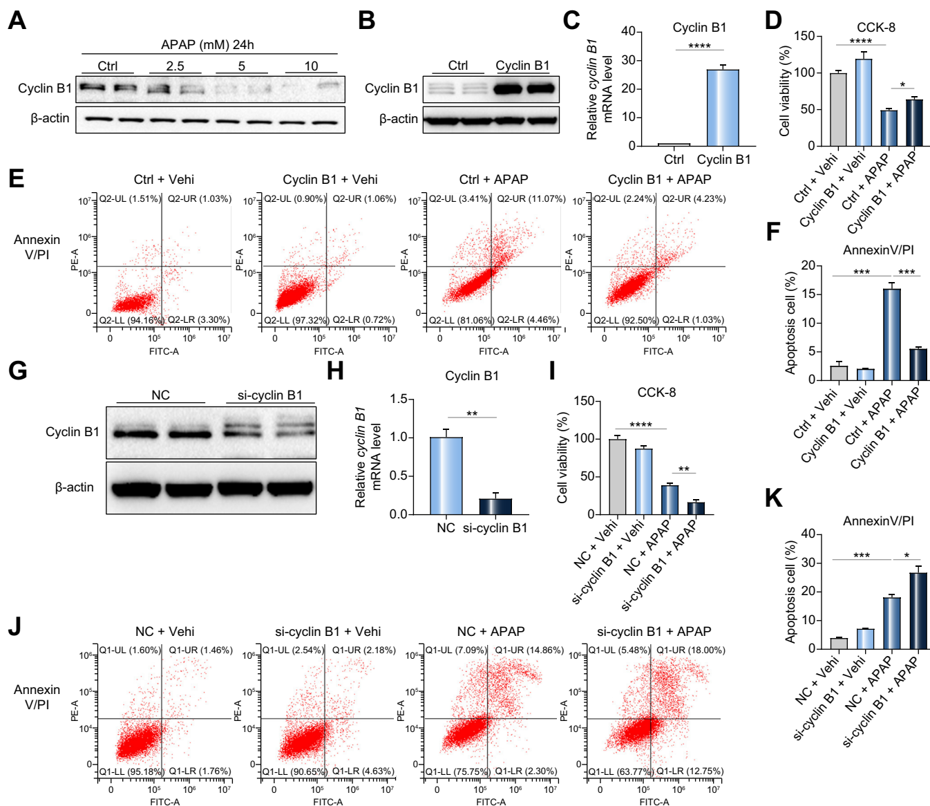
Fig. 6. Effects of cyclin B1 modulation on hepatocyte damage caused by APAP in vitro . (A) Cyclin B1 protein decreased dose-dependently in HepaRG cells treated with APAP for 24 h, n = 4. (B, C) Western blot analysis and RT-PCR displaying the overexpression efficiency of cyclin B1 in HepaRG cells, n = 3–4. (D) Cell viability of HepaRG cells in different groups measured by a CCK-8 assay, n = 6. (E, F) Flow cytometry analysis and quantification of HepaRG cells after FITC Annexin V staining, n = 3. (G, H) The efficiency of si-cyclin B1 (cyclin B1 siRNA) in HepaRG cells was examined by a Western blot analysis and RT-PCR, n = 3–4. (I) Cell viability of HepaRG cells in each group by a CCK-8 assay, n = 6. (J, K) Degree of cell damage as shown by FITC Annexin V staining and the corresponding quantification, n = 3. Experimental design: cells were transfected with si-cyclin B1 or cyclin B1 plasmids for 24 h, followed by APAP or vehicle treatment for 24 h. All values are represented as the means ± SEM. Significant differences were analysed using a 1-way ANOVA or Student t test, * p < 0.05, ** p < 0.01, *** p < 0.001, **** p < 0.0001. APAP, acetaminophen; Ctrl, control; CCK-8, cell counting kit 8; NC, negative control; n.s., no significance; PI, propidium iodide; si, small-interfering; Vehi, vehicle.
