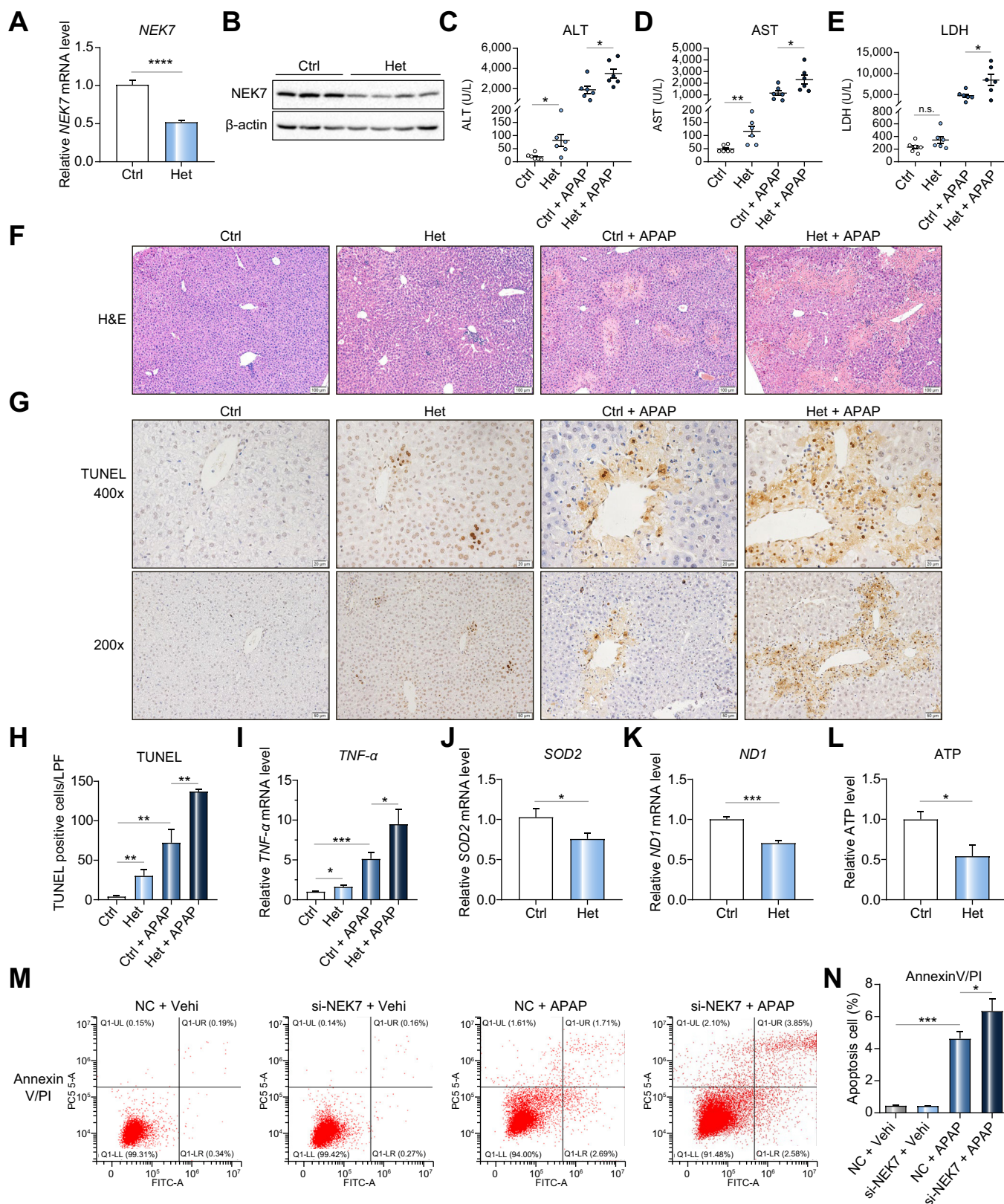
Fig. 3. Conditional knockdown of hepatocyte NEK7 exacerbates APAP-induced ALI. (A, B) Levels of NEK7 protein and mRNA in livers from control mice and Het mice. (C–E) Levels of ALT, AST, and LDH in the serum from each group of mice, n = 6. (F) Representative images of H&E-stained liver sections from each group; scale bars, 100 μm. (G) TUNEL staining of liver sections; scale bars, 20 μm for 400×, 50 μm for 200×. (H) Quantification of positive cells in liver sections stained by TUNEL, n = 3. (I–K) mRNA levels of inflammatory gene ( TNF-α ), antioxidant gene ( SOD2 ) and mitochondrial gene ( ND1 ), n = 5–6 per group. (L) Hepatic levels of total ATP in control and Het mice, n = 6 per group. (M, N) Flow cytometry analysis and quantification of HepaRG cells after FITC Annexin V staining, n = 3. All
