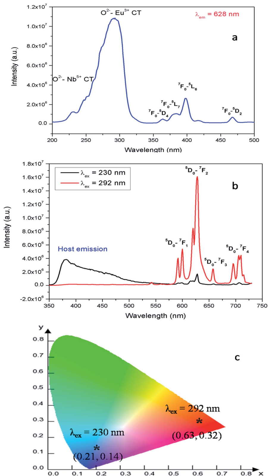
Fig. 5 (a) Photoluminescence excitation and (b) emission spectra of Eu:LNO recorded at room temperature and (c) the corresponding CIE color co-ordinates.
