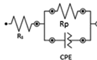
Fig. 4 Randle's equivalent circuit for fitting EIS spectra.
