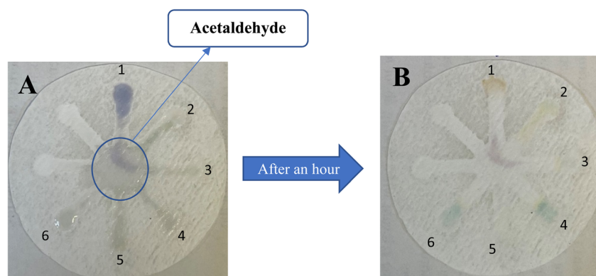
Fig. 9 (A) Photographic images of the microfluidic paper-based calorimetric chemo sensor for evaluation of capillary: AgNPs and colored TMB solution and AgNWs (zone 1–2), AgNWs and colored TMB solution and AgNWs (zone 3–4), AgNPs-Cit and colored TMB solution and AgNPs-Cit (zone 5–6). (B) Photographic images of prepared paper after an hour.
