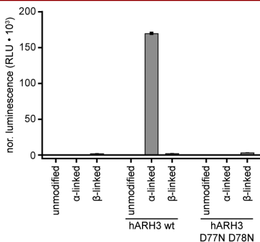
Figure 1. Analysis of the stereospecificity of hARH3. ADPr released in the ARH3 reaction was converted into AMP using hNUDT5 and subsequently measured using the AMP-Glo assay (Promega). Control reactions were carried out both in absence of hARH3 as well as using a catalytically inactive hARH3 mutant (D77N D78N). The data were normalized to reactions containing only hNUDT5 and represent triplicate measurement \pm SD.
