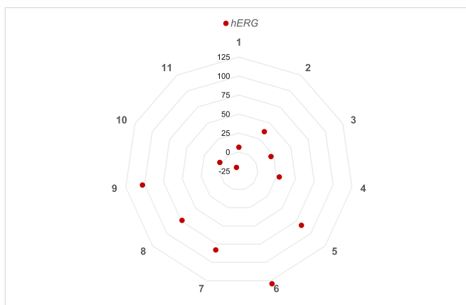
Fig. 5. hERG liability of new thymimimetics. % Inhibition of hERG. See Table 1 for further details.
