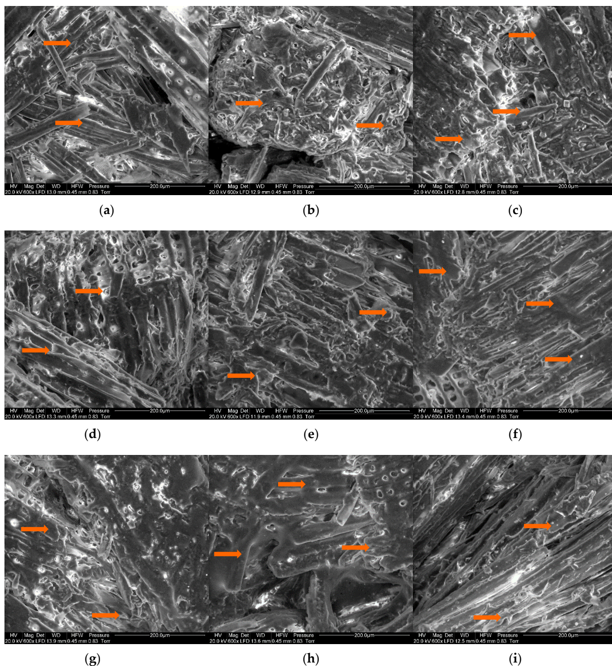
Figure 6. Scanning electron microscope images of lignocellulosic composites with (a) PLA12, (b) PLA15, (c) PLA20, (d) PCL12, (e) PCL15, (f) PCL20, (g) PS12, (h) PS20, (i) UF12; zones covered by binder indicated by arrows.
