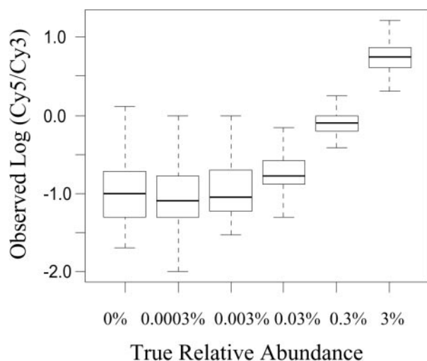
Figure 4. Quantification of species in complex mixtures ('Dilution Pools'). True relative abundance is compared with observed \log(\text{Cy5}/\text{Cy3}) ratio for the 101 species with 1 or more species-specific probes. The x -axis corresponds to the six different relative abundance levels used in this experiment. The y -axis shows the distribution of observed \log(\text{Cy5}/\text{Cy3}) ratios for species at the specified relative abundance level. When more than one probe was available for a given species, we averaged the \log(\text{Cy5}/\text{Cy3}) ratios across all available probes (2–5 probes per species). Box-whisker plot format: box spans the 25% quantile to the 75% quantile surrounding the median; 'whiskers,' extend to span the full dataset excluding outliers; outliers are defined as points beyond 3/2 the interquartile range from the edge of the box.
