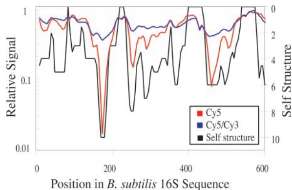
Figure 2. Variation in signal intensity across B. subtilis SSU Sequence. Hybridization of identical Cy5 and Cy3-labeled B. subtilis rRNA to overlapping probes tiling along the B. subtilis SSU rDNA sequence illustrates variation in signal intensity across perfectly matched sequences. Cy5 and Cy5/Cy3 ratio are both normalized to the maximum across the entire tiled region. Self-structure is measured as the length of the longest hairpin. Red, Cy5; blue, Cy5/Cy3; and black, self structure.
