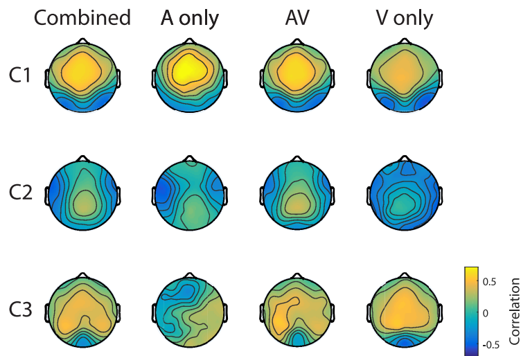
Figure 5. The forward model for the three most correlated components of neural activity. Each column represents the forward model (correlation between surface electrodes and component activity) obtained using either all stimuli together (combining responses across all subjects, left) or different stimulus presentations (A Only, middle-left; AV, middle-right; V Only, right). Each row represents a different component in descending order from most correlated (top) to least correlated (bottom; C1–C3). Color indicates the correlation between each scalp electrode and the component.
