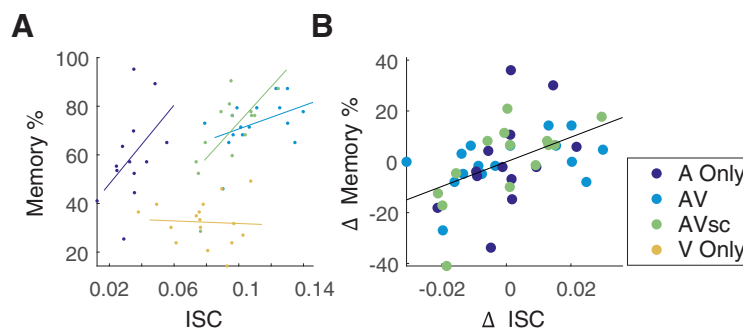
Figure 4. Relationship between neural ISC and memory performance. A , Memory accuracy for auditory information increases with ISC in all conditions in which the auditory narrations were heard (A Only, AV, and AVsc), but not when it was missing (V Only). Each point indicates an individual subject’s ISC (Eq. 2) and memory. B , Same as A , but here, to control for the modality effect, mean values across subjects were subtracted from ISC and memory performance for each subject in that stimulus condition. Only conditions with performance significantly above chance are used.
