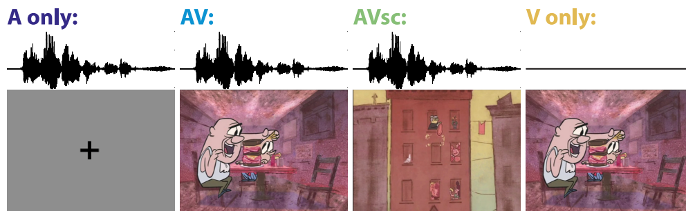
Figure 1. Illustration of the behavioral task. Subjects were exposed to one of five conditions: A Only, AV, AVsc, V Only, or No Stim (not shown). The sound clip represented by the waveform is “...and he would buy me a hotdog the size of my head...” Three weeks after stimulus presentation, and without prior warning, subjects were asked to complete an on-line questionnaire with 72 four-alternative forced-choice questions. The question asked about this segment of the stimulus was “What would Rocco do with the narrator when they went for walks?” Answer options were as follows: “a. Buy him a hot dog; b. Buy him a milkshake; c. Buy him candy; d. Tell him stories.” Still images from “Sundays at Rocco’s,” a StoryCorps animated short produced by Lizzie Jacobs and Mike Rauch, reproduced here with permission from StoryCorps.
