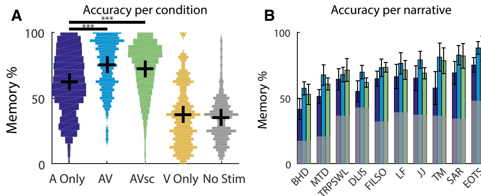
Figure 2. A, B. Memory performance for different stimulus modalities ( A ) and different narratives ( B ). A , Note that exposure to the visual stimuli (V Only, yellow) yields performance no better than chance performance (No Stim, gray). In addition to mean and SE (represented by the black horizontal and vertical lines, respectively), we also present the histogram of the distribution of accuracy values. B , For each narrative (for titles see Materials and Methods), performance is shown for A Only (purple), AV (blue), AVsc (green), and chance (No Stim, gray). Error bars represent the SEM across questions ( N = 72 in A ; N = 5-9 in B ). *p < 0.05 , **p < 0.01 , ***p < 0.001 .
