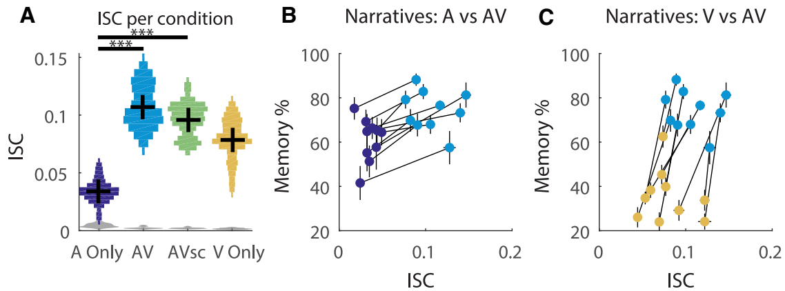
Figure 3. ISC A Only (purple), AV (blue), AVsc (green), and visual (V Only, yellow) stimuli. The full distribution of the ISC values are indicated by the width of the histogram bars for each condition, and gray indicates the distribution of the chance level of correlation for each modality. ISC is calculated using the sum of the three largest correlated components elicited by the presentation of the narrative (Eq. 1). Error bars (vertical lines) represent the SEM across subjects. * p < 0.05 , ** p < 0.01 , *** p < 0.001 . B, C , The multisensory boost in memory and ISC occurs for all 10 narratives. The different presentation conditions for each narrative, corresponding to separate groups of subjects, are connected with a line, and SEs across subjects are represented as horizontal and vertical bars for ISC and Memory %, respectively.
