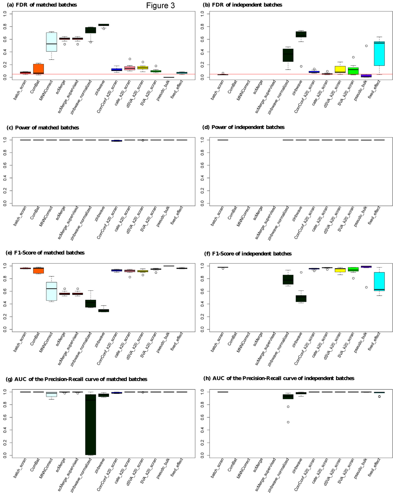
Fig. 3. FDR and power from the simulation of the large sample size and large group effects. a) FDR of matched batches; b) FDR of independent batches; c) power of matched batches; d) power of independent batches; e) F1-score of matched batches; f) F1-score of independent batches; g) AUC of the Precision-Recall curve of matched batches; h) AUC of the Precision-Recall curve of independent batches. The FDR, power, F1-score, and AUC of each method is plotted as a boxplot based on replications. For the FDR, the redline is the nominal threshold of 0.05. A large deviation from this line indicates either inflation or deflation of the FDR.
