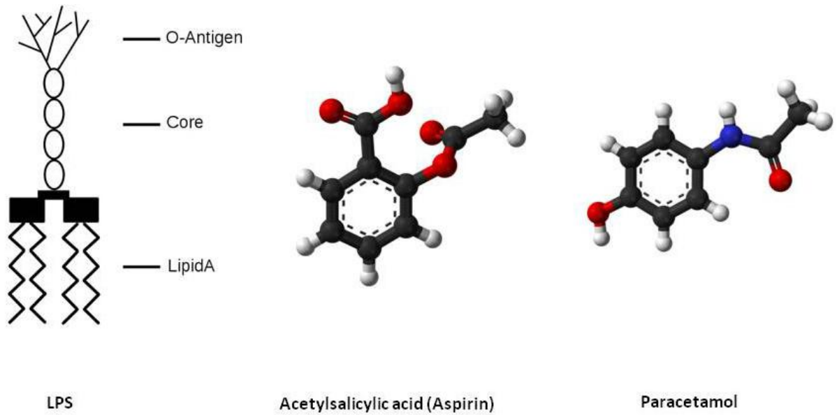
FIGURE 2. Exogenous pyrogens and antipyretic drugs. Molecular models of the exogenous pyrogens LPS and the antipyretic medications acetylsalicylic acid (aspirin) and paracetamol.
