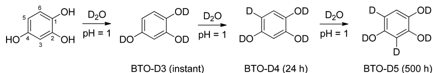
Figure 1. (a) Decomposition of BTO (TCI) in D 2 O (0.125 M) as a function of time under different conditions (acidic: pH 1, basic: pH 10) monitored by 1 H NMR via the signal of the 5-Ar-H compared with an internal standard. (For the illustration, lines are added, obtained through fitting a second-order exponential decay.) (b) Series of 1 H NMR spectra of BTO in acidic (H 2 SO 4 ) D 2 O. Relative decrease in different signal integrals compared with integrals at t 0 for different aromatic protons of (c) BTO and (d) 1. (e) Repeat of spectra series of BTO (Aldrich) in acid (H 2 SO 4 ) and D 2 O on a short time scale. (f) Relative decrease in different signal integrals compared with integrals at t 0 for different aromatic protons of BTO on a shorter time scale.
