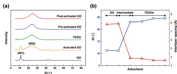
Fig. 5 Diffraction pattern (a) and the corresponding between 2\theta and interlayer spacing of graphene-based materials (b).
