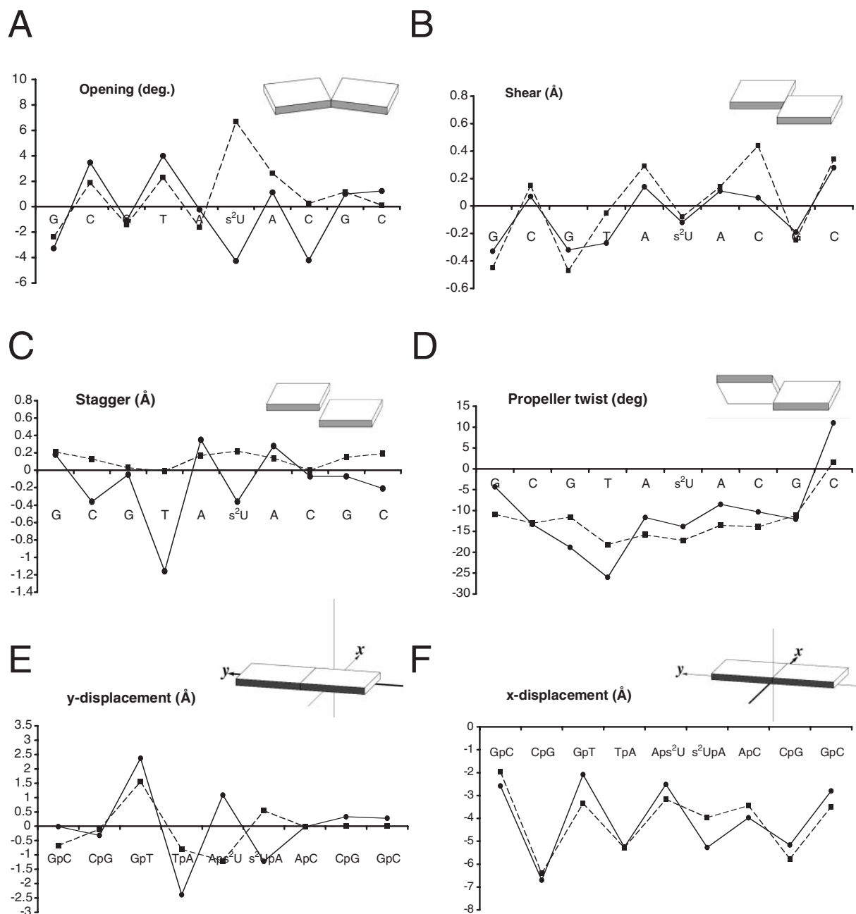
Figure 5. Local inter-base parameters (A) 'opening', (B) 'shear', (C) 'stagger' and (D) 'propeller twist', and local base-pair helical parameters (E) 'y-displacement' and (F) 'x-displacement' in the m 5 s 2 Umoe- (filled circles, thin solid lines) and m 5 Umoe-modified decamer duplexes (filled squares, dashed lines). All parameters were calculated with the program 3DNA (36) and a cartoon of the particular parameter is shown at the upper right in each panel.
