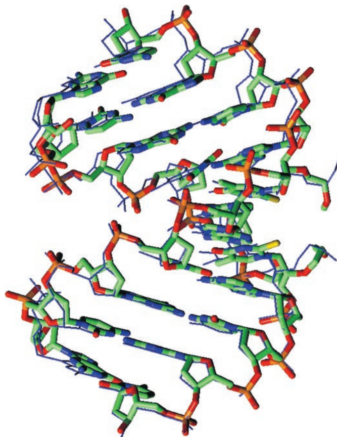
Figure 4. Overall conformation of the m^5s^2U_{moe} -modified decamer (atoms are colored green, blue, red, orange and yellow for carbon, nitrogen, oxygen, phosphorus and sulfur, respectively) compared with the m^5U_{moe} -modified reference duplex (thin blue lines). The view of the A-form duplexes is across the major (top) and minor grooves (bottom) and the 5'-terminal G1 and G11 residues are located at the top left and bottom left, respectively. 2'- O -Substituents are jutting into the minor groove and 2-sulfur atoms highlighted in yellow. The reduced kink into the major groove in the m^5s^2U_{moe} -modified decamer between the tetramer 5'-G1pC2pG3pT4:3'-C20pG19pC18pA17p and the hexamer 5'-pA5p( m^5s^2U_{moe} 6)pA7pC8pG9pC10:3'-( m^5s^2U_{moe} 16)-pA15pT14pG13pC12pG11 is clearly visible.
