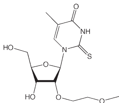
Figure 1. Structure of 2'- O -[2-(methoxy)ethyl]-2-thiothymidine ( s^2m^5Umoe ).
