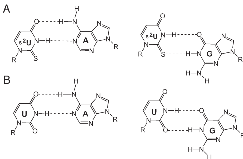
Figure 2. Pairing of U and s^2U with A and G. (A) Diagram illustrating s^2U base-pairing with both A and G; s^2U favors A over G. (B) Diagram illustrating the lack in specificity with uridine; U binds with similar affinity to both A and G.
