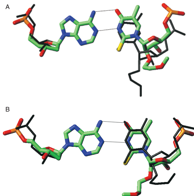
Figure 6. Effects of the 2-thio modification on the geometry of m^5s^2Umoe:A base pairs. (A) Superimposition of the m^5s^2Umoe6:A15 (colored by atom) and m^5Umoe6:A15 (black lines) base pairs, illustrating base opening in the m^5s^2Umoe:A base pair. (B) Superimposition of the A5:m^5s^2Umoe16 (colored by atom) and m^5s^2Umoe6:A15 (black lines) base pairs, illustrating the nearly identical orientations of the C2(A) and S2( m^5s^2Umoe ) atoms in the two pairs. The views are approximately along the normal to the base planes and Watson-Crick hydrogen bonds are drawn as thin solid lines.
