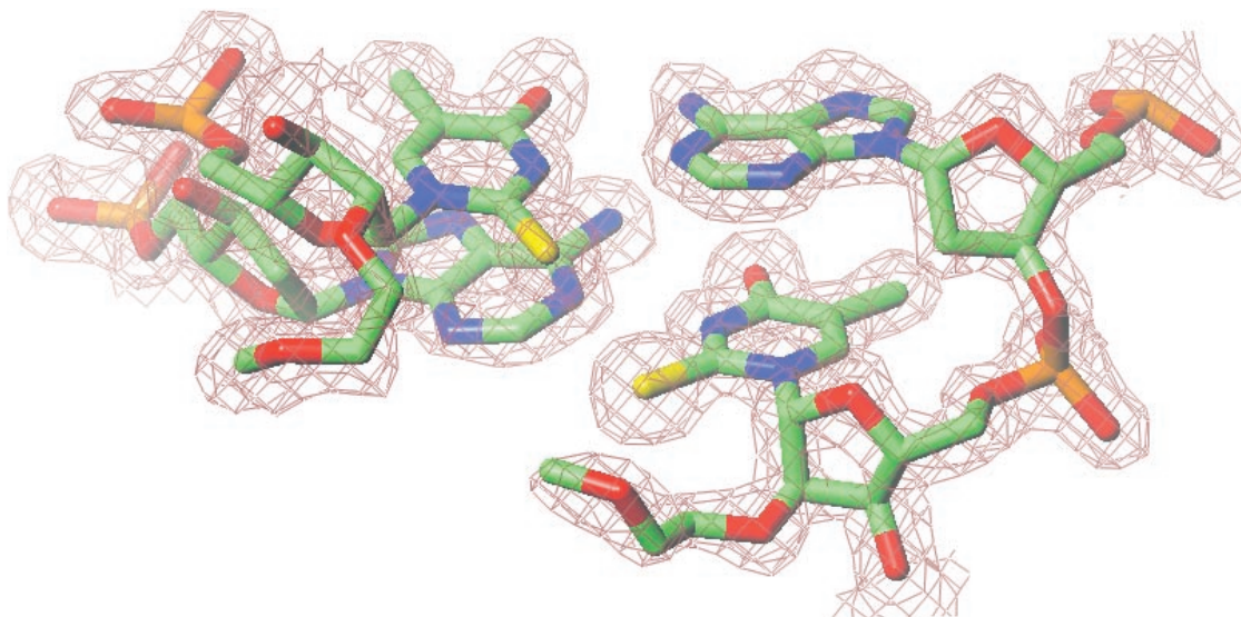
Figure 3. Example of the final sum ( 2F_o - F_c ) Fourier electron density ( 1\sigma threshold) around the base-pair step (A5)p( m^5s^2Umoe6 ):(A15)p( m^5s^2Umoe16 ). The view is into the minor groove with 2'-O-MOE substituents in the foreground ( m^5s^2Umoe6 , left, and m^5s^2Umoe16 , right), and atoms are colored green, blue, red, orange and yellow for carbon, nitrogen, oxygen, phosphorus and sulfur, respectively.
