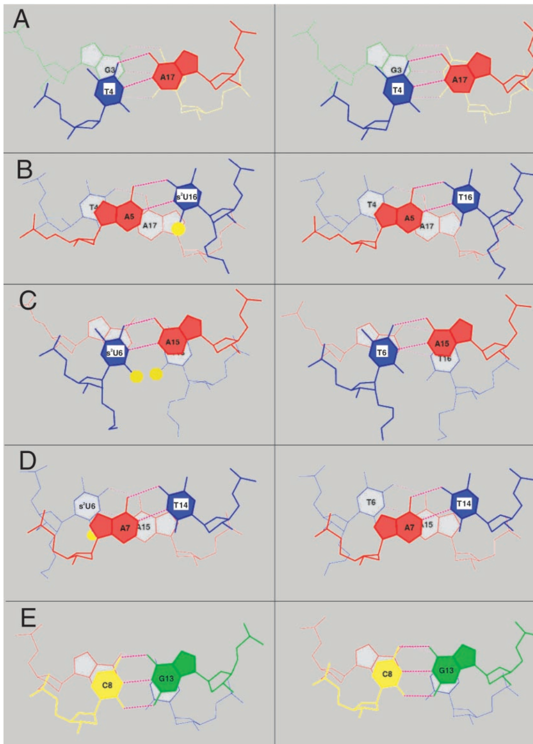
Figure 7. Improvement of stacking interactions as a result of the 2-thio modification. Panels on the left show stacking interactions in the m^5s^2Umoe -modified duplex and panels on the right show stacking interactions at the corresponding steps in the m^5Umoe -modified reference duplex. Base-pair steps (A) (G3)p(T4):(A17)p(C18), (B) (T4)p(A5):(m 5 s 2 Umoe16)p(A17), (C) (A5)p(m 5 s 2 Umoe6):(A15)p(m 5 s 2 Umoe16), (D) (m 5 s 2 Umoe6)p(A7):(T14)p(A15) and (E) (A7)p(C8):(G13)p(T14). G, C, A and T are colored green, yellow, red and blue, respectively, and sulfur atoms are highlighted as yellow spheres. The figures were generated with the program 3DNA (36).
