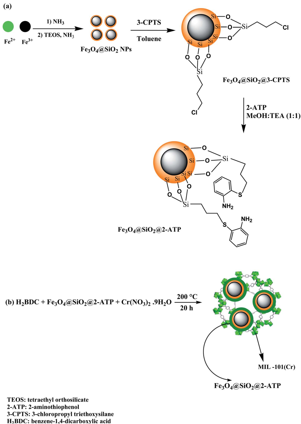
Fig. 1 A scheme for the synthesis of (a) Fe 3 O 4 @SiO 2 @2-ATP nanoparticles, and (b) MIL-101(Cr)/Fe 3 O 4 @SiO 2 @2-ATP nanocomposite.
