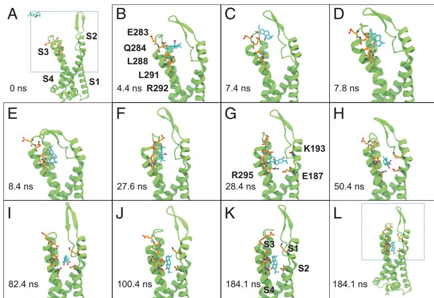
Fig. 8. MD simulations reveal the mechanism of pisiferic acid binding to the VSD of Kv1.1. (A) Expanded view of the S1–S4 helices and pisiferic acid in bulk solvent. Dashed lines correspond to the area in (B). (B) Close-up view of pisiferic acid. The ligand contacts and interacts with E283 and Q284 at the S4 helix. (C) Pisiferic acid shifts and enters a solvent-exposed cavity in the VSD. (D–F) L288, L291, and R292 coordinate the ligand as it reaches the binding pocket and (G) adopts a metastable configuration coordinated by K193, R295, and E187. (H and I) The ligand flips prior to settling in the stably bound pose (J), and remains in this conformation for the remainder of the simulation (K). (L) Expanded view of the ligand bound to the VSD.
