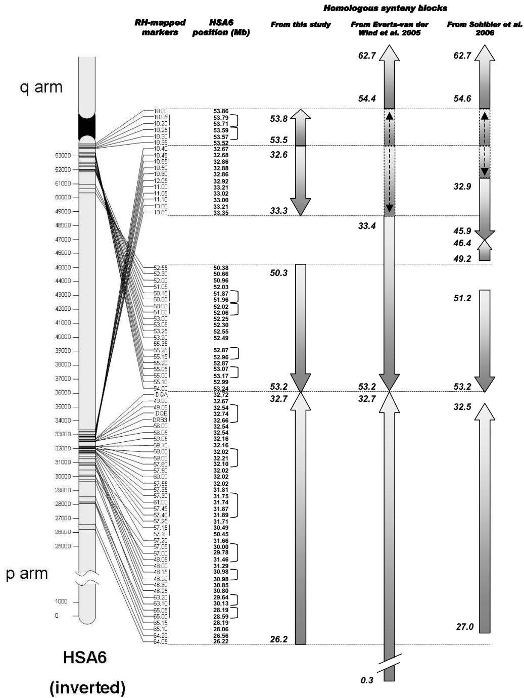
Figure 3 Homologous syntenic blocks in cattle and human. Details about human homologs identified for RH-mapped markers used in this study. To the left, the BoLA RH-mapped markers are presented in their homologous HLA positions, with the corresponding megabase position of the human homolog listed to the right. Brackets indicate markers clustered by the RH analysis. These clustered markers have been assigned to the same cR position and therefore can be flipped with equal likelihood; as a result, caution should be exercised when considering these markers as part of an inversion. To the right, arrows indicate locations and orientations of homologous syntenic blocks in relation to human, determined by this study, [14], and [29]. Proposed extensions of HSBs are represented as lighter-colored blocks with dotted edges; orientation is indicated by arrows within the blocks.
