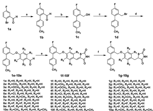
Scheme 1 Reagents and conditions: Synthesis of target compounds 1g–10g . (a) 4-Tolylboronic acid, \text{Pd}(\text{PPh}_3)_4 , \text{Na}_2\text{CO}_3 , toluene, ethanol, \text{H}_2\text{O} , 80 °C, 12 h, 81%; (b) \text{NaBH}_4 , \text{CH}_3\text{OH} , THF, 0 °C, 1 h; (c) \text{PBr}_3 , \text{CH}_2\text{Cl}_2 , 0 °C, 1 h, 58% (two-steps); (d) \text{K}_2\text{CO}_3 , DMF, rt., 12 h; 71–86% (e) \text{NH}_4\text{OAc} , AcOH, 100 °C, 12 h; (f) biacetyl dioxime, \text{NaBH}_4 , \text{CoCl}_2 , NaOH, \text{H}_2\text{O} , 0 °C, 52–64% (two-steps).
