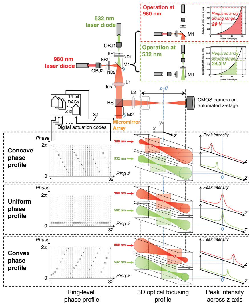
Fig. 7 Schematic diagram of the optical test setup, performed measurements and drive electronics. For two distinct laser source wavelengths (532 and 980 nm), multiple phase masks corresponding to different target depths along the optical z axis were applied by driving the rings of the micromirror array with 32 DACs. Mirror M1 was employed to switch between laser sources. Mirror M2 was employed to alternate the reflection between the micromirror array and plain mirror to assess the focusing efficiency \eta . A CMOS camera mounted on an automated z -stage was employed to acquire z -stack images across the full focusing range. For a given convex or concave phase mask, operation at 980 nm resulted in greater focusing power and a larger spot size compared to operation at 532 nm (OBJ: objective, SF: spatial filter, ND: neutral density filter, M: mirror, L: lens, and BS: beamsplitter)
