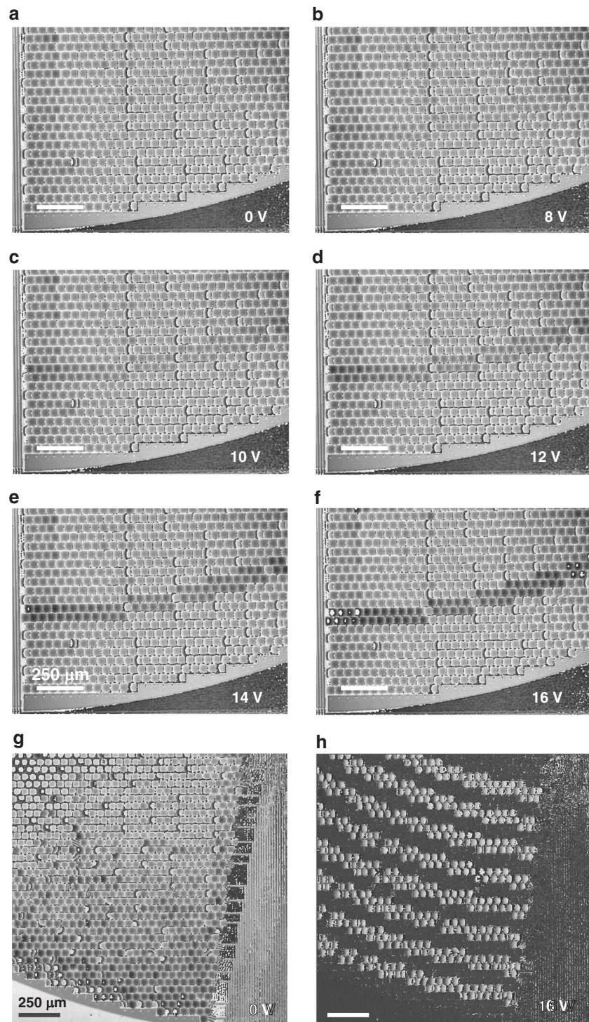
Fig. 6 Phase reconstruction images obtained via digital holographic microscopy demonstrating ring-level actuation of the array (all scale bars are 250 \mu\text{m} ). a–f A single ring (#28 of 32 from the centre) was actuated in increasing steps with applied voltages of 0, 8, 10, 12, 14 and 16 V. g, h Alternating rings (#17, #19, #21, #23, #25, #27, #29 and #31 from the centre) were concurrently actuated with an applied voltage of 16 V. g Phase reconstruction before actuation. h Phase difference after actuation
