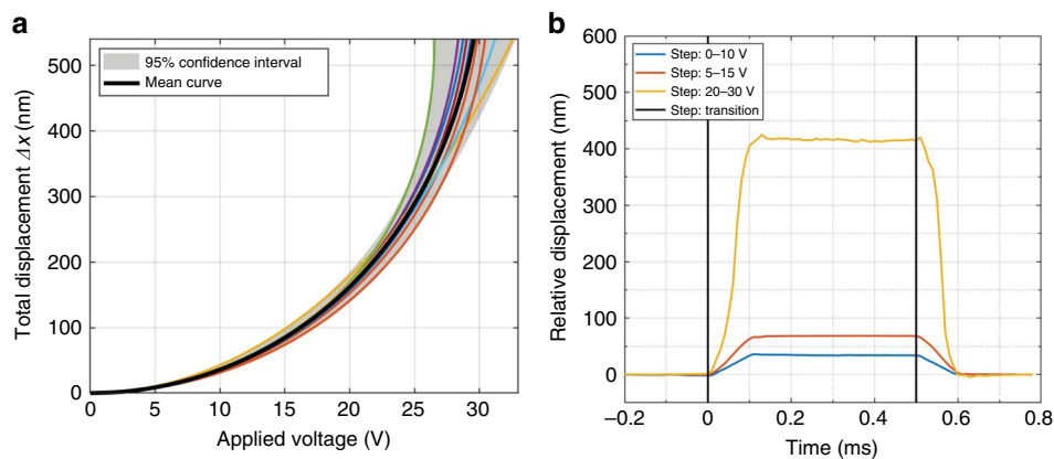
Fig. 5 Pixel-level steady-state and dynamic transduction characterization results obtained via digital holographic microscopy. a Measured steady-state displacement vs applied voltage. The coloured curves correspond to individual pixel measurements from various pixels across arrays. b Mean settling behaviour of pixels measured stroboscopically by applying 1 kHz square wave voltage signals with a 10 V step and varying the offsets for increasing ranges of displacement
