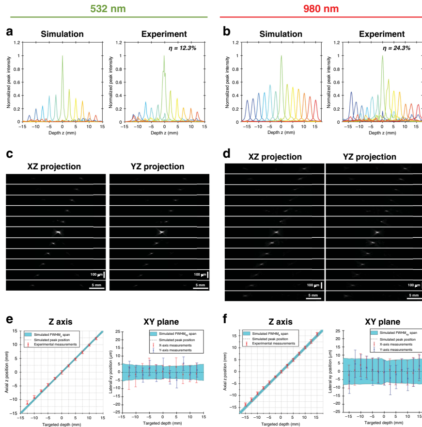
Fig. 8 Optical focusing performance results. a, b Simulated and experimental results of the peak intensity values projected along the optical axis for 532 nm ( a ) and 980 nm ( b ) sources. Each coloured line corresponds to a distinct applied phase mask, and the efficiency \eta is included as an inset. c, d Lateral projections of the acquired Z-stacks along the XZ plane and YZ plane for all applied phase masks with 532 nm ( c ) and 980 nm ( d ) sources. The scales for the lateral dimensions (X and Z) differ from the Z-axis scales as indicated by the provided scale bars. e, f Spot size and position measurements along the X, Y and Z dimensions compared against the simulated values for 532 nm ( e ) and 980 nm ( f ) sources. The spans of the measurement bars and simulation envelopes correspond to the spot size values measured as full width at half maximum. X-shaped measurement markers correspond to the peak intensity position along z for left side plots and the peak intensity distance from optical axis for right side plots
