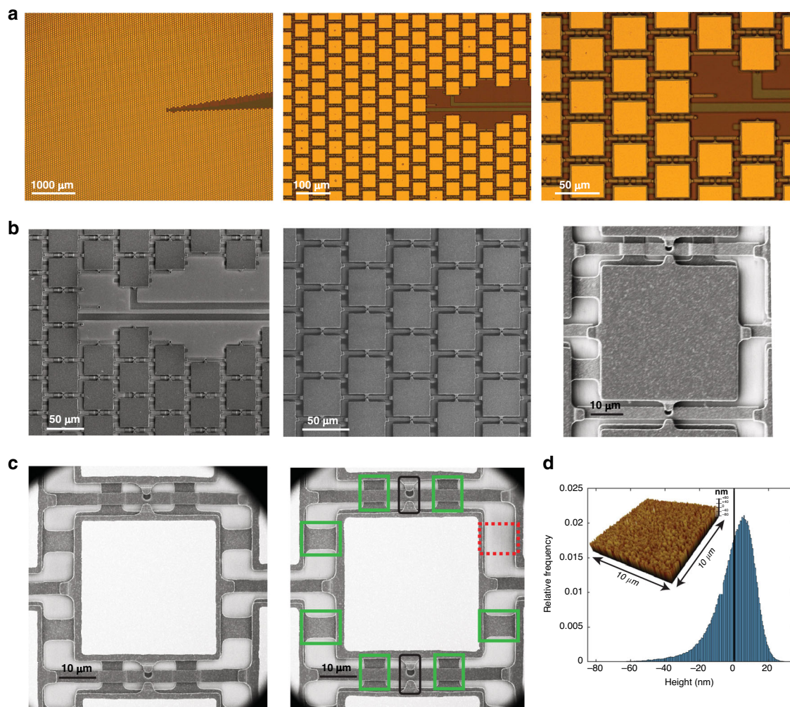
Fig. 3 Fabrication images of the produced array. a Optical microscopy images of the array centre at various levels of magnification. b Scanning electron microscopy (SEM) images of the array prior to metallization postprocessing at various levels of magnification. c SEM images of two different pixels after metallization. Electrical wiring across pixels for grouped drive is achieved via 8 potential connections between fixed bottom electrodes at the Polysilicon 0 layer, which can be added (green boxes, right image) or removed (red box, right image) in accordance with the partitioning geometry. For each pixel, two Polysilicon 2 juts (black boxes, right image) hanging over the anchors of adjacent suspension beams serve as gap stop structures preventing electrode contact from electrostatic pull-in during operation. d Topography histogram of the deposited reflective gold layer as measured by atomic force microscopy (AFM). The heights are measured per 50 nm × 50 nm region; histogram bin sizes are 0.5 nm. The top-left inset is a sample 2-dimensional topography plot across an area of 10 μm × 10 μm
