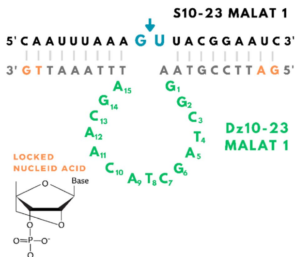
Fig. 1 Secondary structure of the 10–23 DNzyme. The figure illustrates the RNA substrate strand in black, the substrate recognition strand of the DNzyme in light gray. The two residues in light blue show the cleavage site. Catalytic core and numbering are shown in green. Orange bases indicate where LNA modifications were introduced in the DNzyme sequence in this study.
