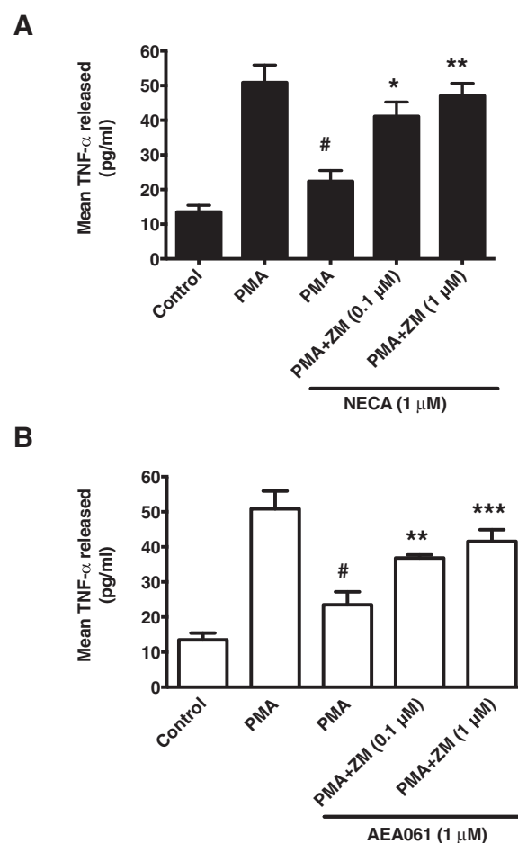
Figure 7 Reversal of AEA061-mediated inhibition of TNF-α production by ZM 241385. Human monocytes were pretreated for 15 min with the A 2a R antagonist ZM 241385 before PMA stimulation (5 ng/ml) and incubation with either the AR agonist NECA (1 μM; A ) or AEA061 (1 μM; B ) for 12 h. TNF-α in the culture medium was quantified by ELISA. # = p < 0.001 PMA versus PMA plus AEA061 or NECA; * = p < 0.05, ** = p < 0.01 *** = p < 0.001 PMA plus AEA061 or NECA with ZM versus without ZM.
