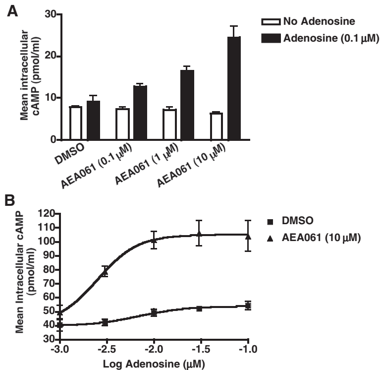
Figure 2 Augmentation of adenosine-mediated activation of the human A_{2a}R ( hA_{2a}R ). (A) AEA061 enhances adenosine-mediated cAMP production by the hA_{2a}R . CHO- hA_{2a}R cells were incubated with adenosine, and AEA061 for 15 min. Mean cAMP levels \pm SEM of a representative experiment is shown ( n = 3 ). (B) AEA061 potentiates both the affinity and the efficacy of adenosine at the hA_{2a}R . CHO- A_{2a}R cells were incubated with AEA061 and varying concentrations of adenosine for 15 min. Mean EC_{50} values of three experiments with SEM were 4.4 \pm 1.3 nM and 1.5 \pm 0.49 nM without and with AEA061 respectively. Increase in E_{max} by AEA061 = 2.1 \pm 0.27 fold.
