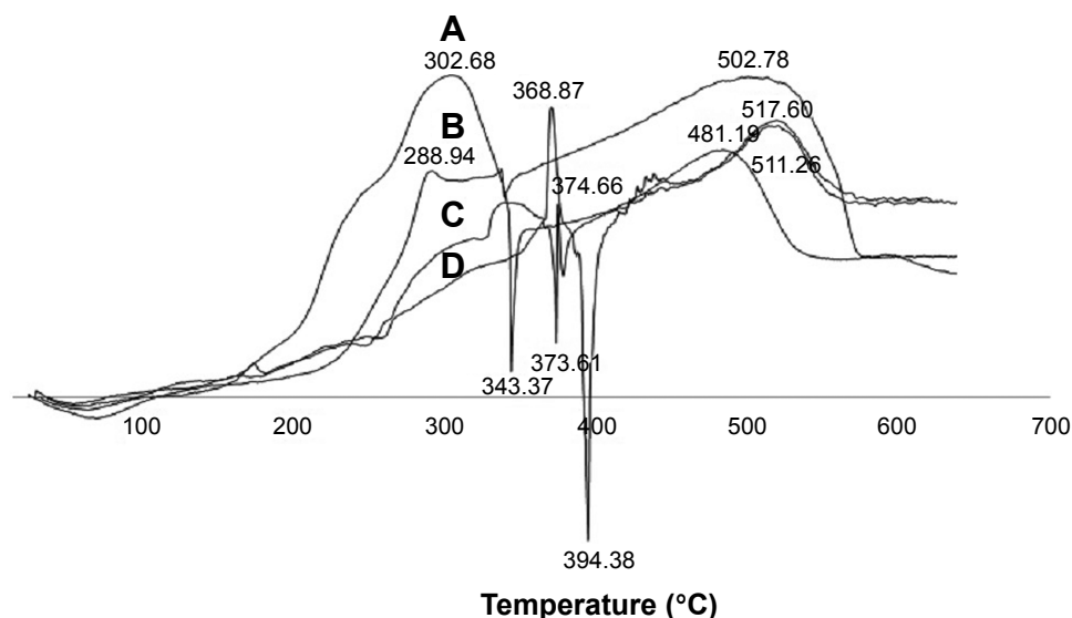
Figure 3 The DSC thermograms of (A) CTS/PL/ \beta -CD microspheres, (B) CTS, (C) PL, and (D) PL/ \beta -CD mixture. Abbreviations: DSC, differential scanning calorimetry; CTS, chitosan; PL, phospholipid; \beta -CD, \beta -cyclodextrin.
