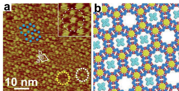
Fig. 4 STM images and proposed model for the TPTA-COR-CuPc host-guest structure at the interface between n -octanoic acid and graphite at room temperature. (a) 60 \times 60 nm 2 , I_{\text{set}} = 378.1 pA, V_{\text{bias}} = 499.9 mV, (b) the proposed molecular model for the TPTA-COR-CuPc host-guest construction.
