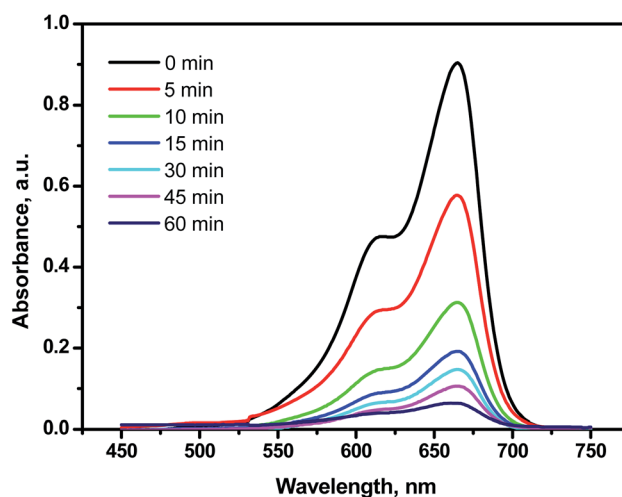
Fig. 10 Time-resolved photocatalytic spectra of MB dye ( 4 \text{ mg L}^{-1} ) upon the treatment with 0.04 \text{ g} of MTPS nanophotocatalyst under the normal day light.
