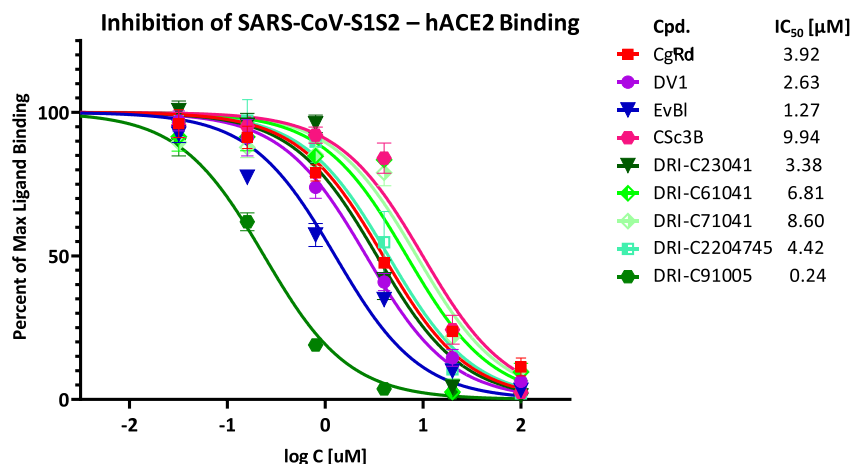
Figure 4. Concentration-dependent inhibition of SARS-CoV-S1S2 binding to ACE2 by representative compounds of the present study. Concentration–response curves obtained for the inhibition of the PPI between SARS-CoV-S1S2 (His-tagged, 1 μg/mL) and hACE2 (Fc-conjugated, 1 μg/mL) in cell-free ELISA-type assay by selected representative dye and nondye compounds. Data and fit as before (Figure 3). Most compounds including several DRI-C compounds show similar activity against SARS-CoV (i.e., SARS-CoV-1) as against SARS-CoV-2 raising the possibility of broad-spectrum activity.
