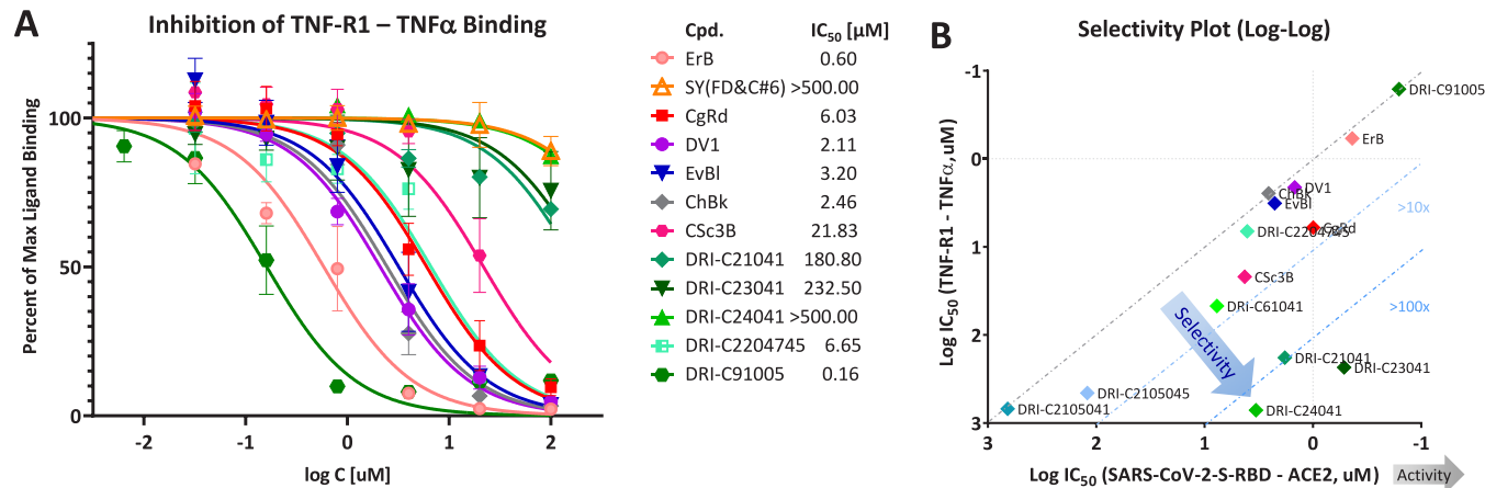
Figure 5. Concentration-dependent inhibition of TNF-R1–TNF \alpha binding by compounds of the present study and corresponding selectivity plot. (A) Concentration–response curves obtained for the inhibition of this important TNF superfamily PPI in similar cell-free ELISA-type assay as used for the CoV-S–ACE2 PPIs to assess selectivity. Data and fit as before (Figure 3). As the IC 50 values indicate, some of the DRI-C compounds showed more than 100-fold selectivity in inhibiting the CoV-S PPI vs the TNF PPI. (B) Selectivity plot comparing inhibitory activity (as quantified by log IC 50 ) against the TNF-R1–TNF- \alpha interaction with that against the desired PPI target (SARS-CoV-2-S-RBD–hACE2). Active and selective compounds are clustered in the lower right corner as highlighted by the trend-indicating arrows.
