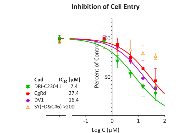
Figure 8. Concentration-dependent inhibition of SARS-CoV-2 pseudovirus (VSV-ΔG) entry into hACE2/Furin expressing host cells by selected compounds. Entry of VSV-ΔG pseudoviruses bearing the SARS-CoV-2 S protein (plus GFP reporters) in ACE2/Furin overexpressing host cells (Vero-E6) was quantified via GFP fluorescence in a live imaging system (Incucyte). CgRd and DRI-C23041 showed concentration-dependent inhibition with IC 50 values consistent with the previous assay (Figure 7), whereas the negative control sunset yellow (SY FD&C #6) showed no significant effect.
