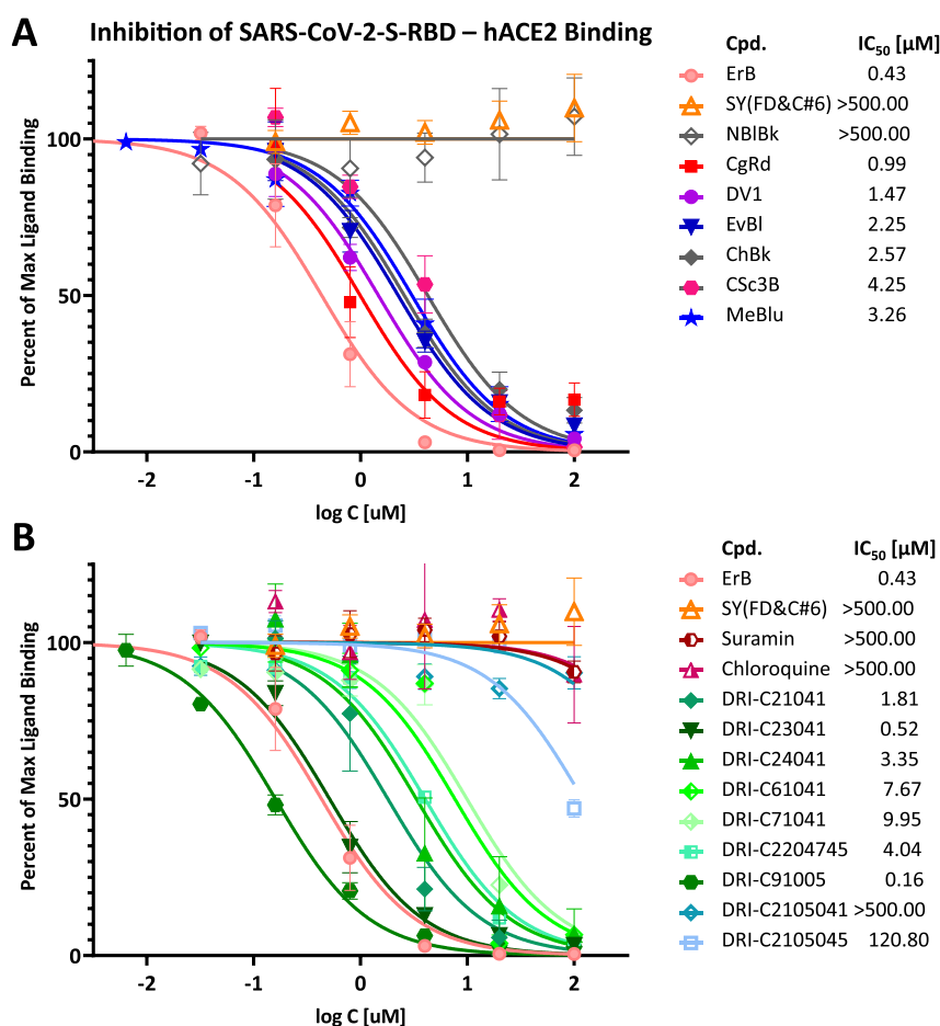
Figure 3. Concentration-dependent inhibition of SARS-CoV-2-S-RBD binding to ACE2 by compounds of the present study. Concentration–response curves obtained for the inhibition of the PPI between SARS-CoV-2-RBD (His-tagged, 0.5 µg/mL) and hACE2 (Fc-conjugated, 1 µg/mL) in cell-free ELISA-type assay with dye (A) and nondye (B) compounds tested. The promiscuous PPI inhibitor erythrosine B (ErB) and the food colorant FD&C yellow no. 6 (sunset yellow, SY) were included as a positive and negative controls, respectively. Data are mean ± SD from two experiments in duplicates and were fitted with standard sigmoid curves for IC 50 determination. Estimated IC 50 's are shown in the legend indicating that while suramin and chloroquine were completely inactive (IC 50 > 500 µM), several of our in-house compounds including organic dyes (CgRd, DV1, and others) as well as proprietary DRI-C compounds (e.g., DRI-C23041, DRI-C91005) showed promising activity, some even at submicromolar levels (IC 50 < 1 µM).
