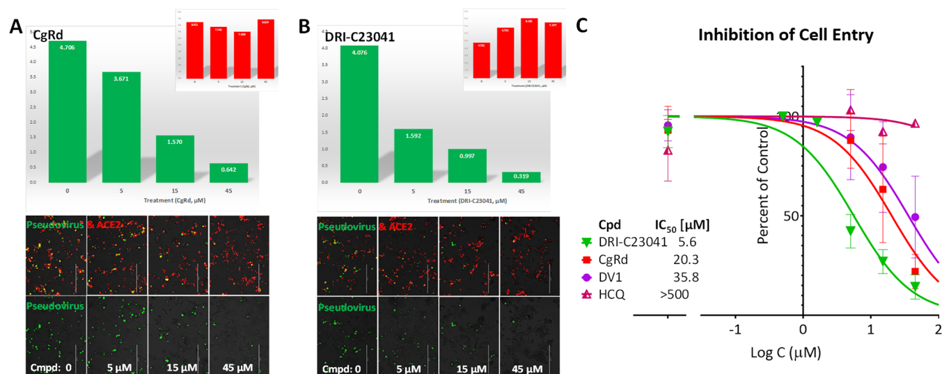
Figure 7. Concentration-dependent inhibition of SARS-CoV-2 pseudovirus entry (BacMam) into hACE2 expressing host cells by selected compounds. Quantification of entry of pseudoviruses bearing the SARS-CoV-2 S protein (plus green fluorescent protein reporters; BacMam-based) in ACE2 (plus red fluorescence)-expressing host cells (HEK293T). Representative images (bottom row) and their quantification for pseudovirus (green) and ACE2 expression (red) using ImageJ (top row) are shown from one experiment for CgRd and DRI-C23041 in (A) and (B), respectively; average data from three experiments fitted with typical concentration–response curves are shown in (C). The amount of green present is proportional with the number of infected cells as green fluorescence is expressed only in pseudovirus infected cells, while amount of red is proportional with the number of ACE2-expressing cells. The organic dye CgRd (A), but especially DRI-C23041 (B) showed concentration-dependent inhibition with activities corresponding to low micromolar IC 50 values, whereas hydroxychloroquine (HCQ) showed no effect (C).
