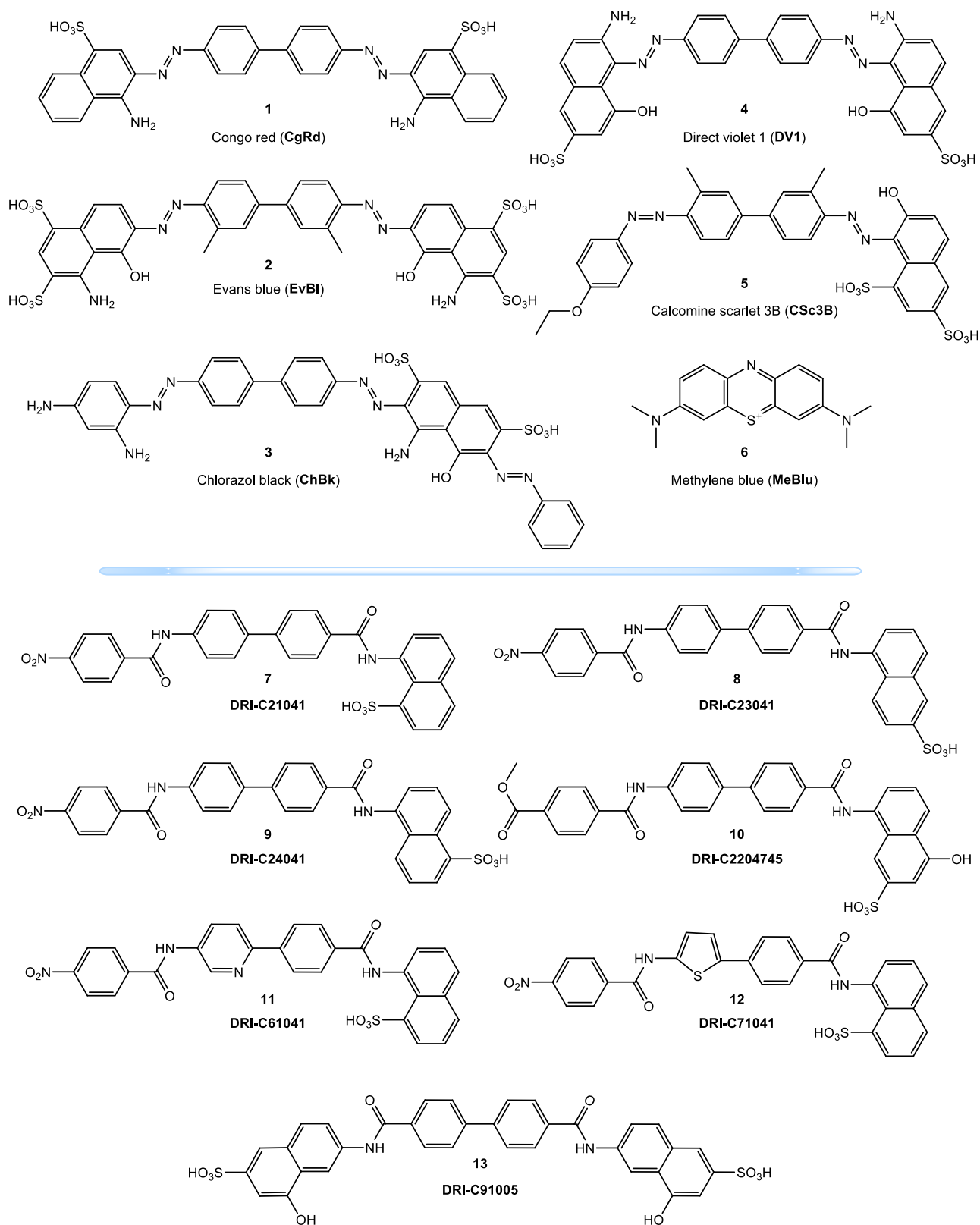
Figure 1. Compounds of the present study. Chemical structures of the organic dye (1–6) and nondye DRI-C compounds (7–13) used in the present study.
