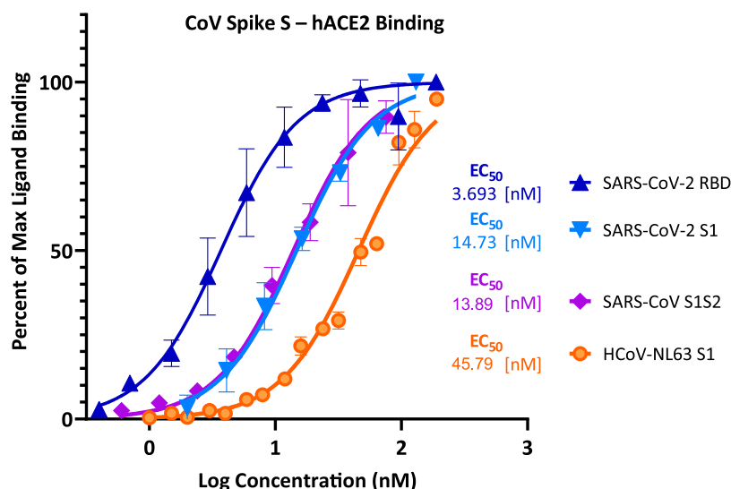
Figure 2. Concentration–response curves for binding of CoV spike protein domains to human ACE2 in cell-free ELISA-type assays. Binding curves and corresponding EC 50 's are shown for SARS-CoV-2 (RBD and S1), SARS-CoV (S1&S2), and HCoV-NL63 (S1). They were obtained using Fc-conjugated hACE2 coated on the plate and His-tagged S1, S1S2, or RBD added in increasing amounts as shown with the amount bound detected using an anti-His–HRP conjugate (mean \pm SD for two experiments in duplicates).
