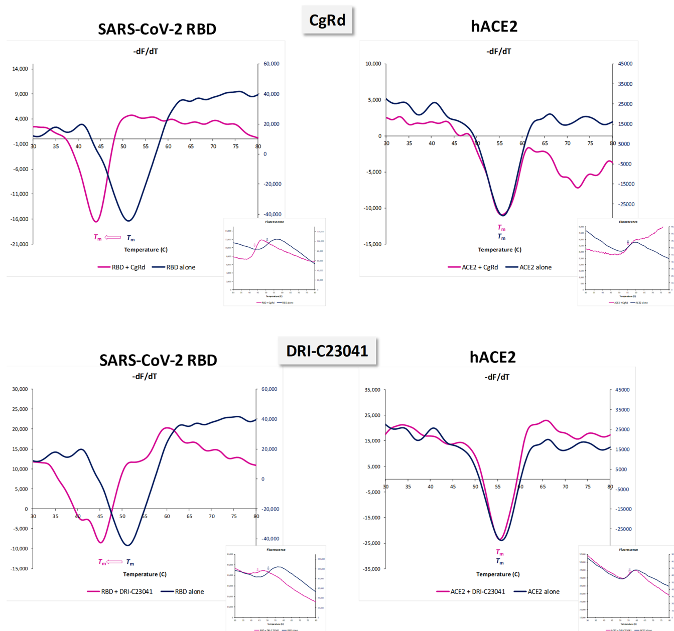
Figure 6. Identification of the binding partner by protein thermal shift. Differential scanning fluorimetry assay indicating SARS-CoV-2 RBD and not ACE2 as the binding partner of the present SMIs compounds. The presence of Congo red (top) or DRI-C23041 (bottom) at 10 \mu M caused clear shifts in the melting temperature of the protein for RBD as indicated by the derivatives dF/dT (left; purple vs blue line), but not for hACE2 (right) (smaller insets are normalized fluorescence F data).
