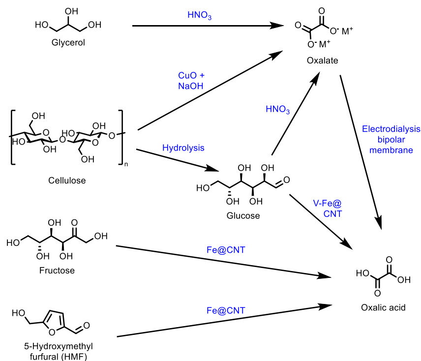
Figure 66. Routes to oxalic acid from sustainable biomass sources, excluding CO 2 and CO.
