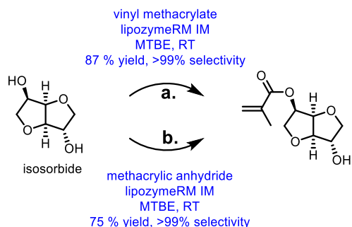
Figure 30. Biochemical approaches to synthesize a monofunctional isoribide methacrylate.
