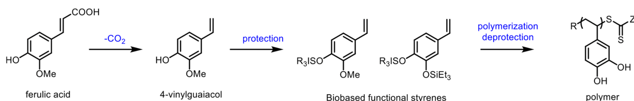
Figure 9. Synthesis, protection and polymerization of bio-based styrenics derived from ferulic acid.
