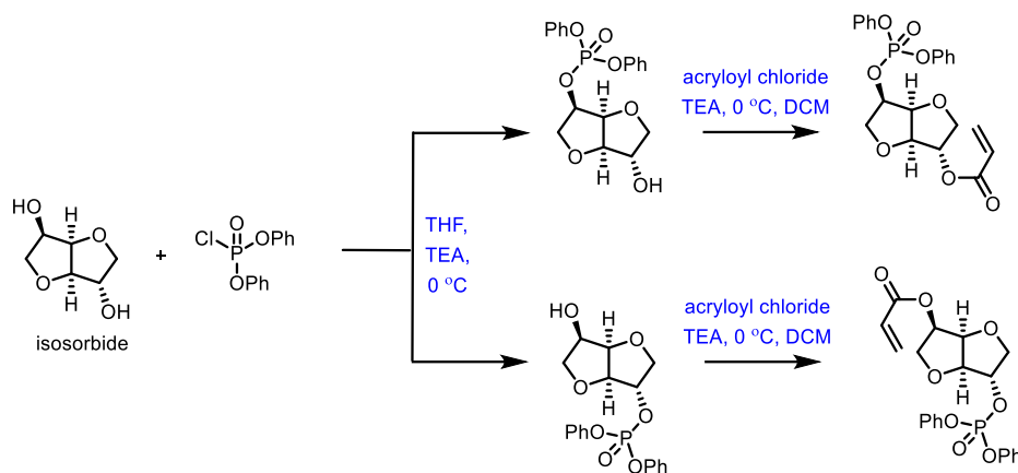
Figure 31. Conversion of isoribide into two isomers of diphenylphosphato acrylates.
