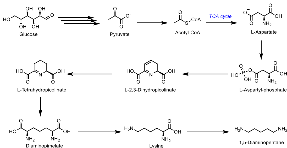
Figure 93. Biotechnological production of 1,5-pentanediamine from glucose, via lysine, where triple arrows indicate multiple steps.
