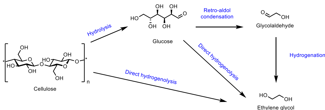
Figure 85. Conversion of cellulose and glucose to ethylene glycol (EG). Cellulose can be converted in a three-step procedure or via direct hydrogenolysis. Glucose is an intermediate of the direct hydrogenolysis pathway and can be used directly as a feedstock for direct hydrogenolysis to EG.
