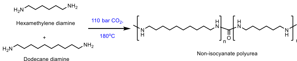
Figure 104. Catalyst-free synthesis of non-isocyanate polyureas (NIPUAs) from the reaction of diamines in supercritical \text{CO}_2 .
