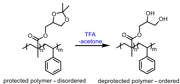
Figure 15. Structures of the protected and deprotected polymers and how it affects the structure of the polymer in solution.
