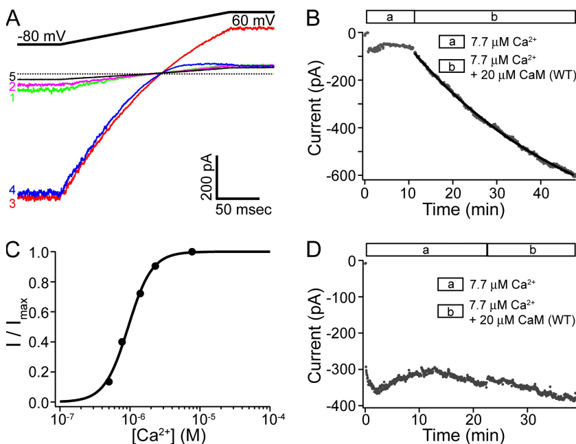
Figure 2. CaM (WT) can recover SK channel activity. (A) Representative current traces with a patch from a CaM (E2Q)-coinjecting oocyte at the following time points: (1) immediately after patch excision; (2) after rundown stabilized; (3) 50 min after the application of 20 \mu\text{M} CaM (WT); (4) the application of solution containing 16 \mu\text{M} \text{Ba}^{2+} ; and (5) finally in \text{Ca}^{2+} -free solution. (B) Average current level at -80 mV measured every 3 s with the patch shown in A during the course of rundown and recovery. Legends in this and later figures show the different solutions that the patch is subjected to. Solid line represents fit with a single-exponential time course ( \tau = 39.7 min). (C) With the same patch shown in A and B, after recovery of SK channel activity with CaM (WT), solutions containing different free \text{Ca}^{2+} concentrations were applied to the patch. Average current level at -80 mV was measured at each concentration, normalized to the maximal value, and plotted as a function of \text{Ca}^{2+} concentration. The dose-response relationship is fitted with the Hill equation: I/I_{\text{max}} = 1/(1+(\text{EC}_{50}/[\text{Ca}^{2+}])^h) , yielding \text{EC}_{50} = 0.94 \mu\text{M} and h = 2.6 . (D) A representative time course of the average current level at -80 mV with a patch excised from an oocyte coinjecting with RNA for SK channels and CaM (WT).
